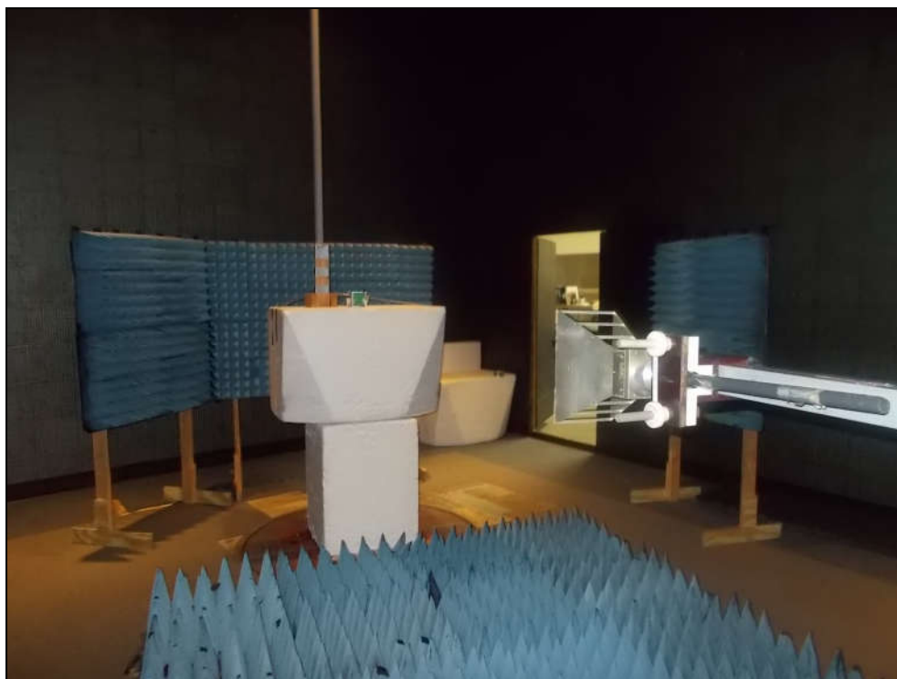
Figure 1: Radiated Emissions – YPOS
