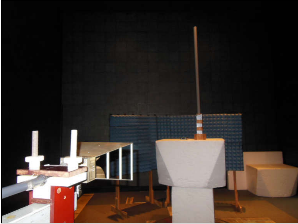
Figure 3: Radiated Emissions – ZPOS
