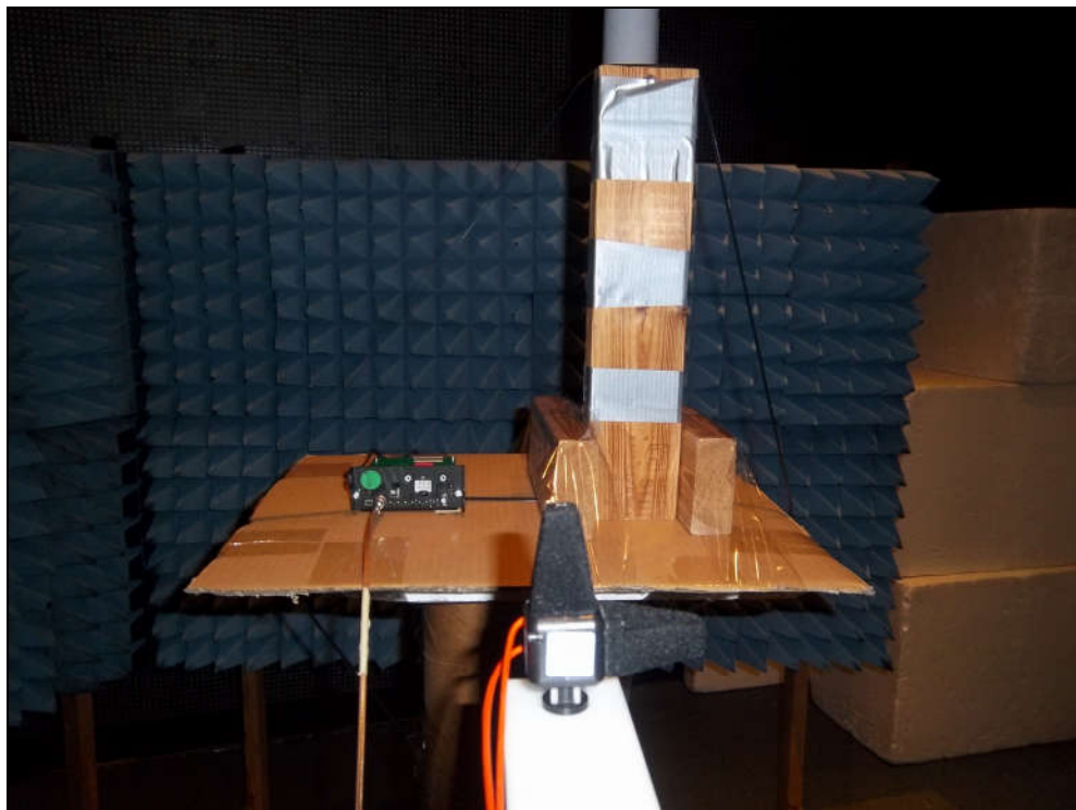
Figure 10: MPE Measurements – ZPOS
