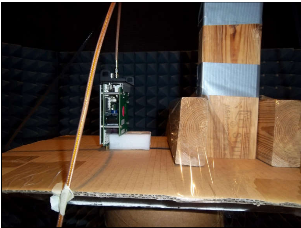
Figure 6: MPE Measurements – XPOS
