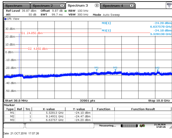
Figure 7.5.2.2-12: CE – OFDM – 600kbps – HCH
