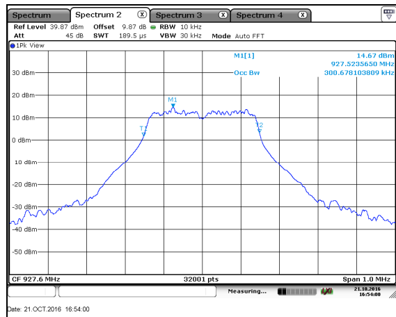
Figure 7.4.4.2-24: 99% BW High Ch – OFDM – 600kbps
