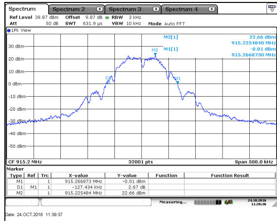
Figure 7.4.4.2-26: 20dB BW Mid Ch – DSSS – 6.25kbps
