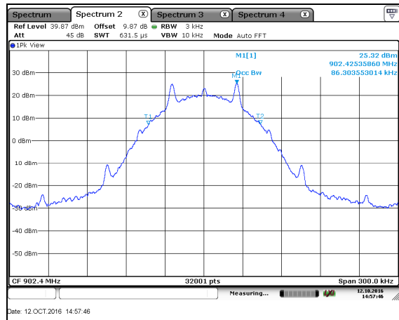
Figure 7.4.4.2-4: 99% BW Low Ch - FSK - 50kbps
