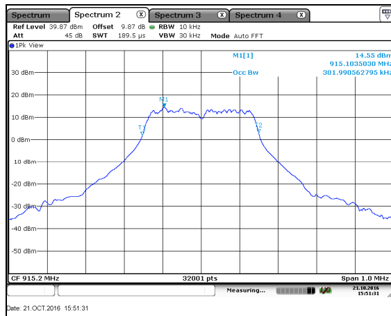
Figure 7.4.4.2-17: 99% BW Mid Ch – OFDM – 200kbps
