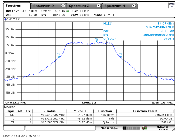
Figure 7.4.4.2-14: 20dB BW Mid Ch – OFDM – 200kbps
