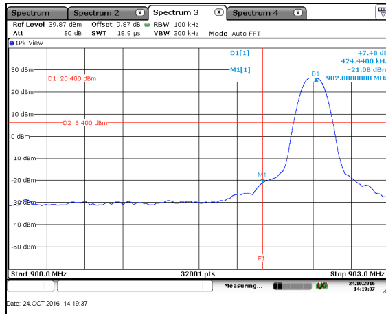
Figure 7.5.1.2-11: Lower BE – DSSS – 12.5kbps
