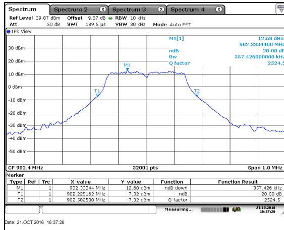
Figure 7.4.4.2-19: 20dB BW Low Ch – OFDM – 600kbps
