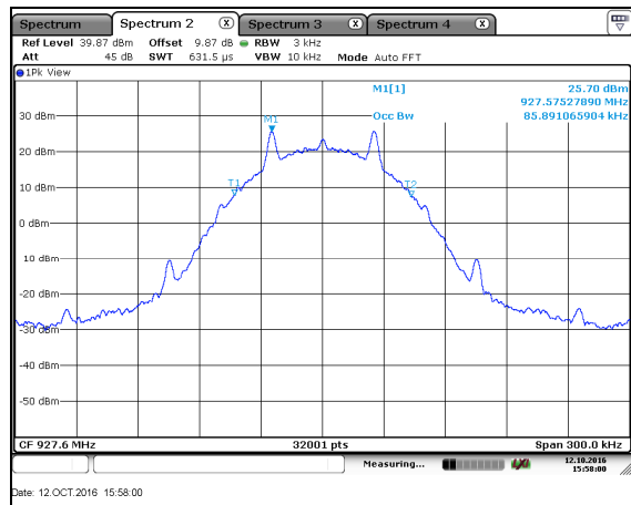
Figure 7.4.4.2-6: 99% BW High Ch - FSK - 50kbps
