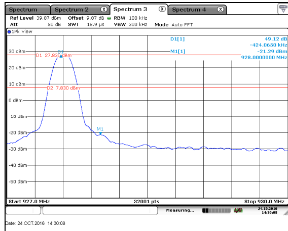
Figure 7.5.1.2-12: Upper BE – DSSS – 12.5kbps
