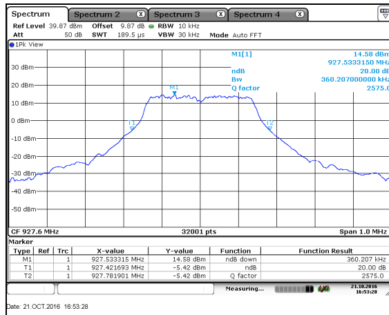
Figure 7.4.4.2-21: 20dB BW High Ch – OFDM – 600kbps
