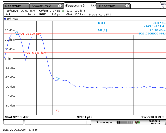
Figure 7.5.1.2-16: Upper BE Hop – FSK – 150kbps
