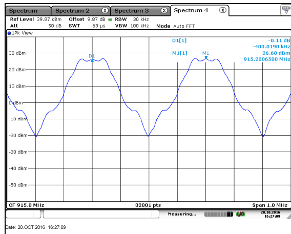
Figure 7.4.1.2-2: Freq. Separation – FSK – 150kbps
