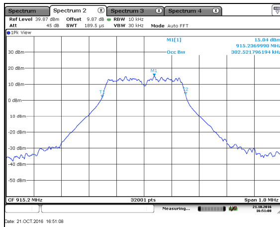
Figure 7.4.4.2-23: 99% BW Mid Ch – OFDM – 600kbps
