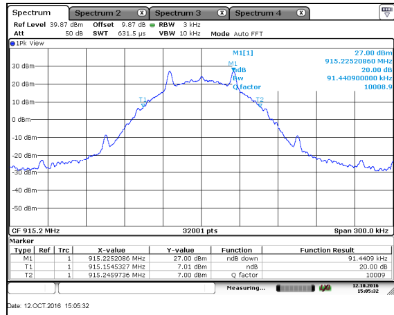
Figure 7.4.4.2-2: 20dB BW Mid Ch - FSK - 50kbps
