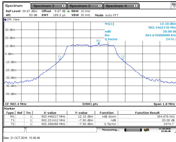
Figure 7.4.4.2-13: 20dB BW Low Ch – OFDM – 200kbps
