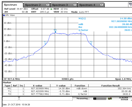
Figure 7.4.4.2-15: 20dB BW High Ch – OFDM – 200kbps
