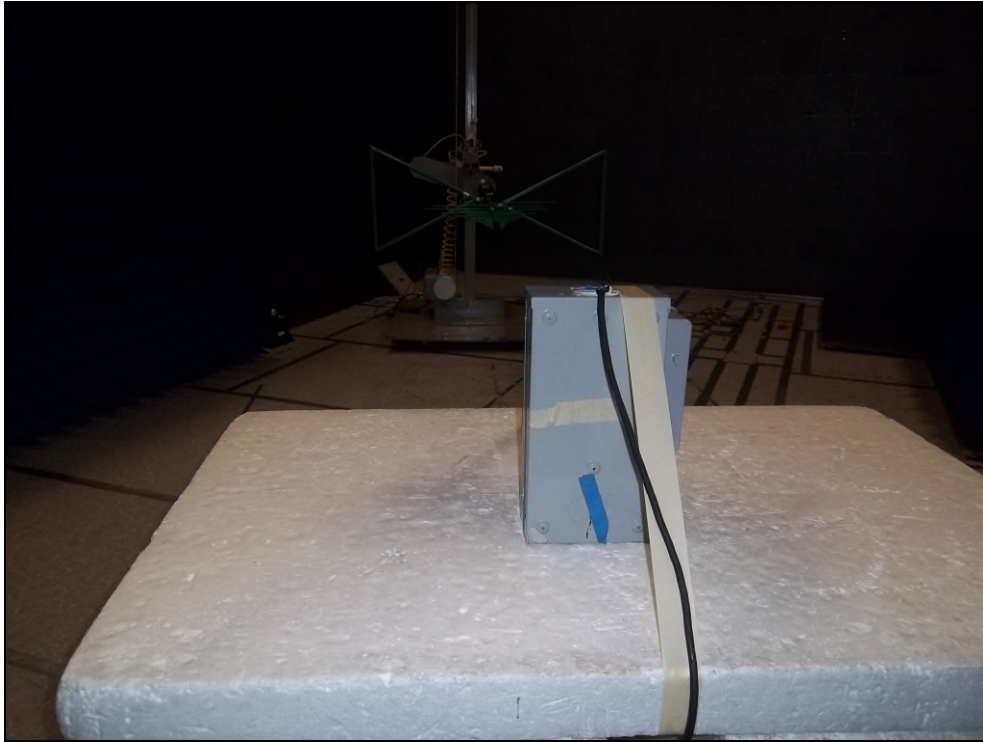
Figure 3: Equipment Under Test – Radiated Emissions <1GHz
