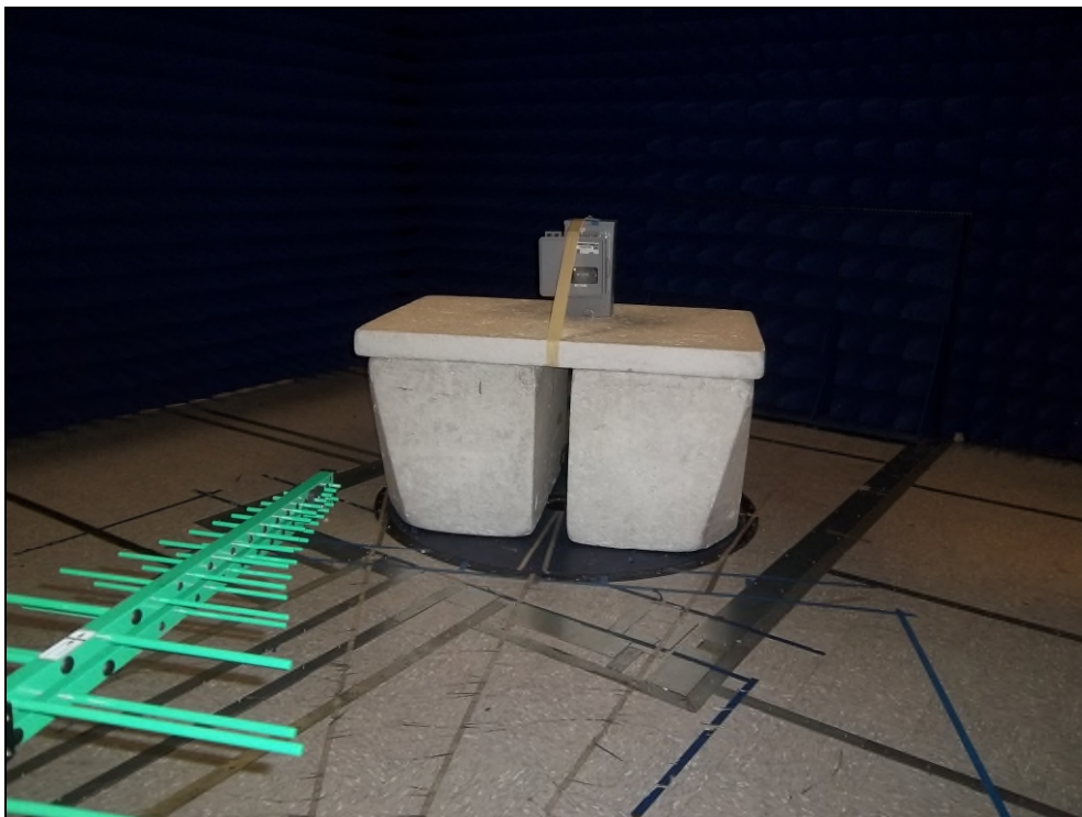
Figure 4: Equipment Under Test – Radiated Emissions <1GHz
