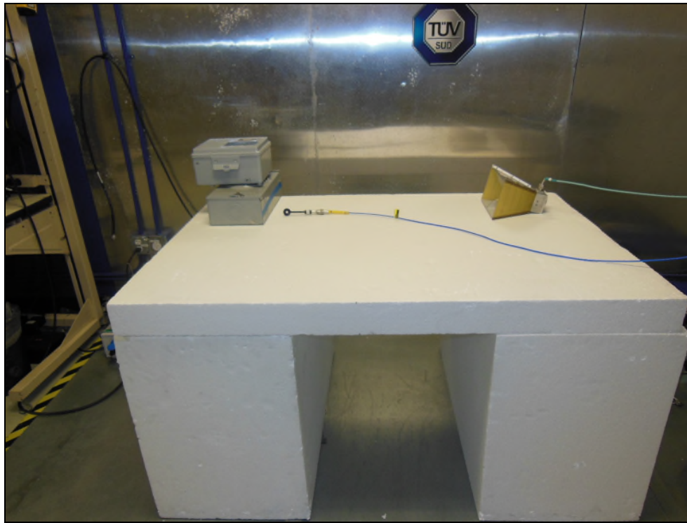
Figure 7: Equipment Under Test – AC Conducted Emissions
