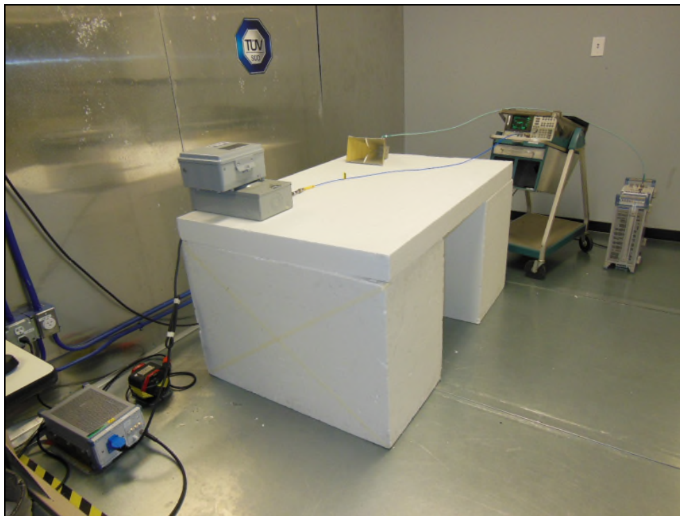
Figure 8: Equipment Under Test – AC Conducted Emissions
