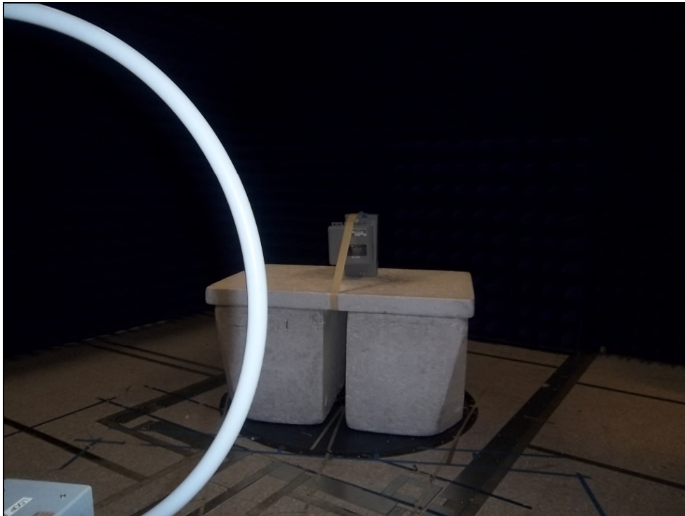
Figure 2: Equipment Under Test – Radiated Emissions <30MHz
