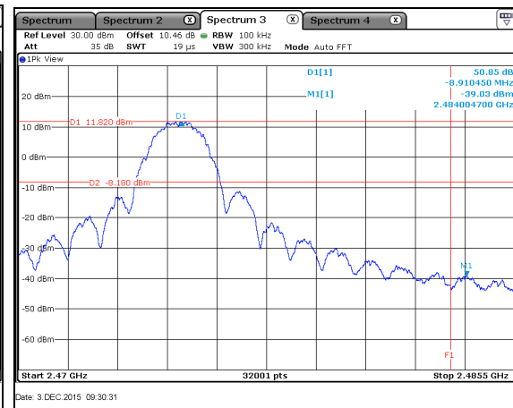
Figure 7.5.1.2-5: Upper Band-edge – CH25
