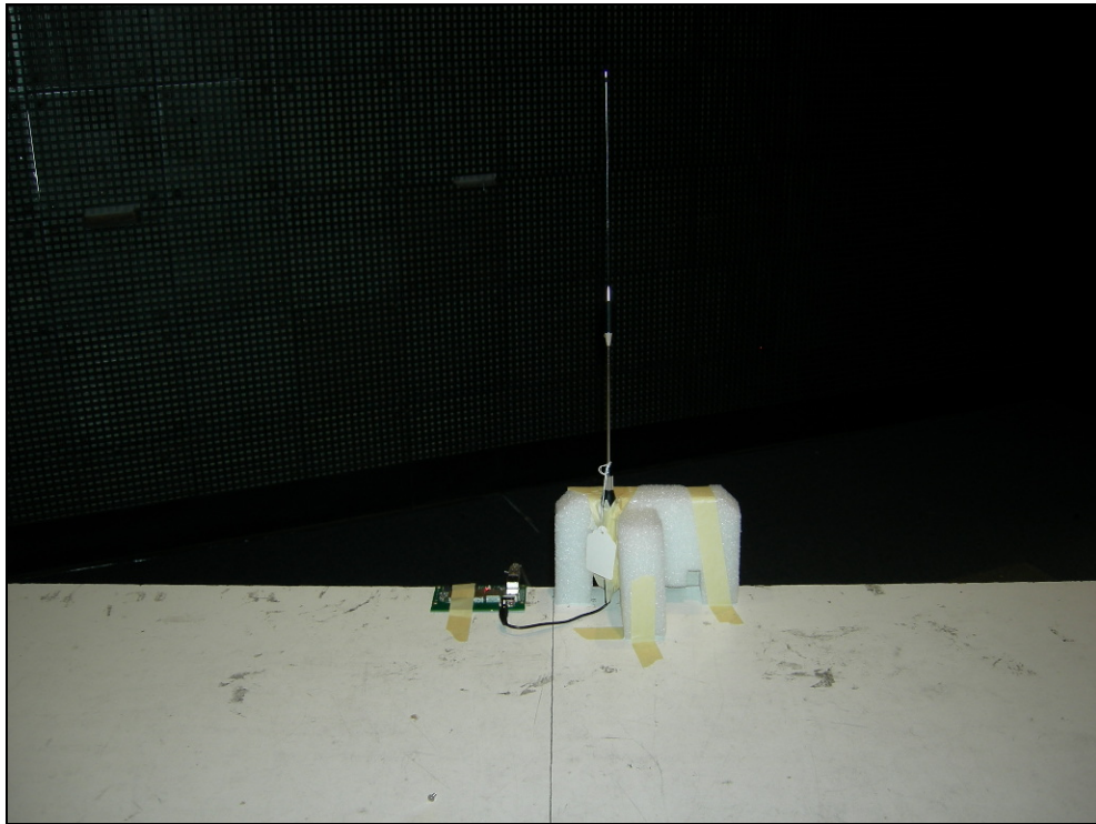
Figure 1: Test Setup Photograph – X-POS – Front View
