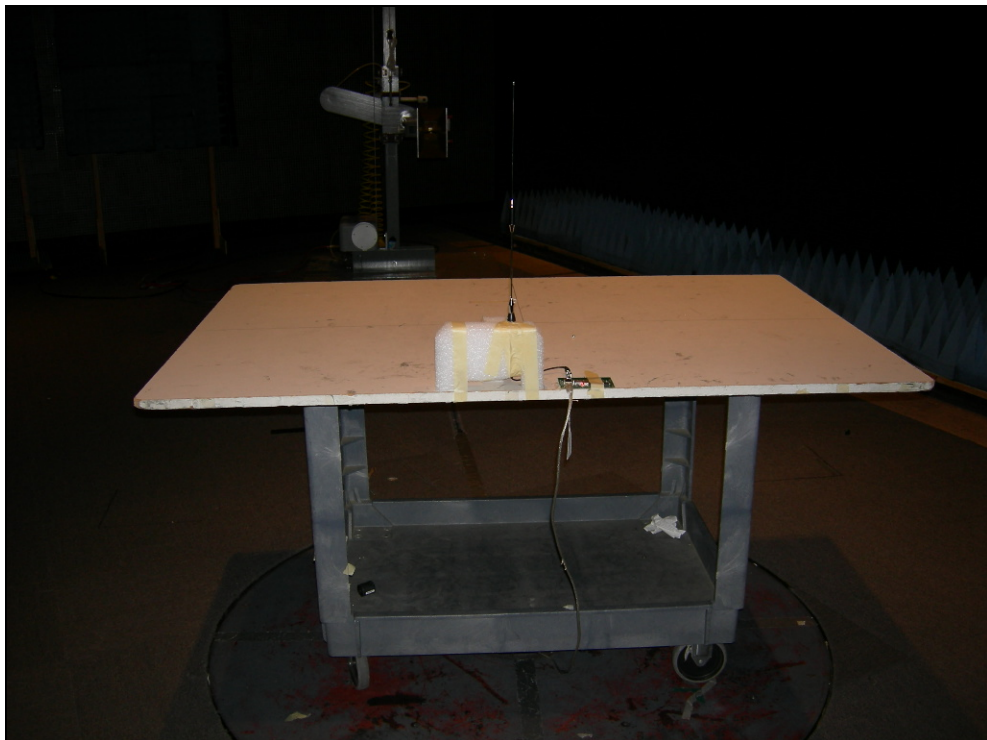
Figure 2: Test Setup Photograph – X-POS – Rear View
