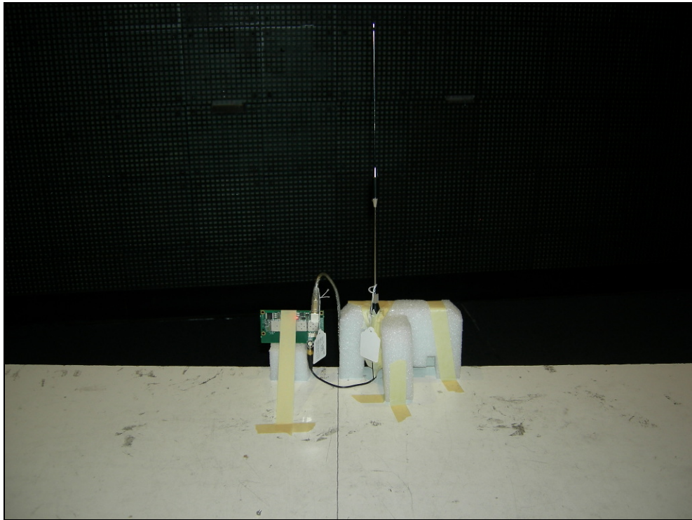
Figure 5: Test Setup Photograph – Z-POS – Front View
