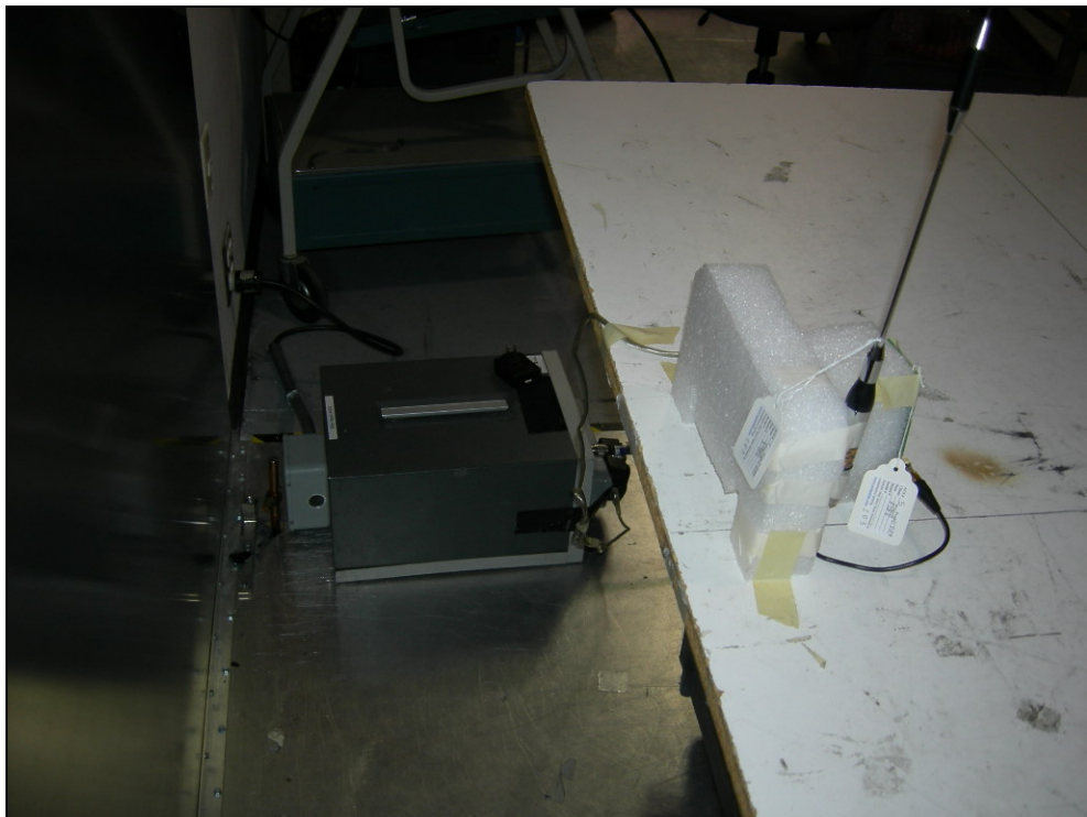
Figure 11: Conducted Emissions
