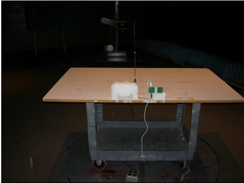
Figure 9: Radiated Emissions – Z-Pos
