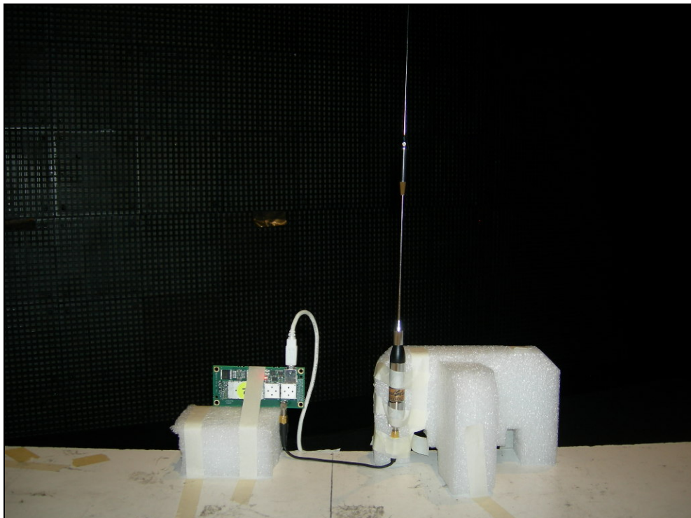
Figure 8: Radiated Emissions – Z-Pos
