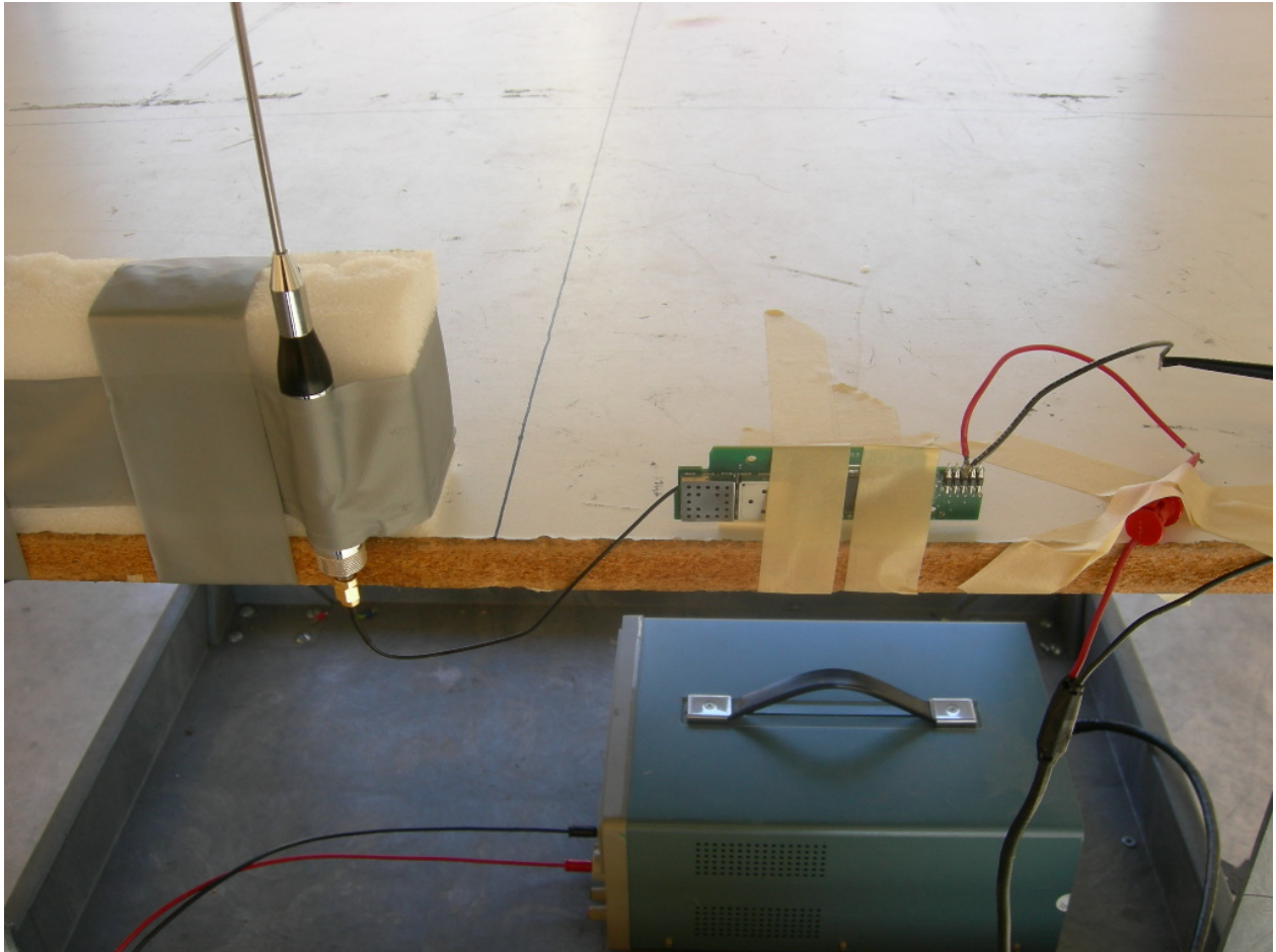
Figure 4: Radiated Emissions – Intentional – Orientation 2
