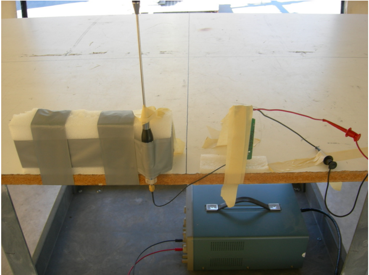
Figure 3: Radiated Emissions – Intentional – Orientation 1
