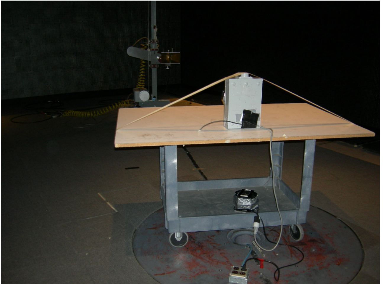
Figure 2: Radiated Emissions - Intentional
