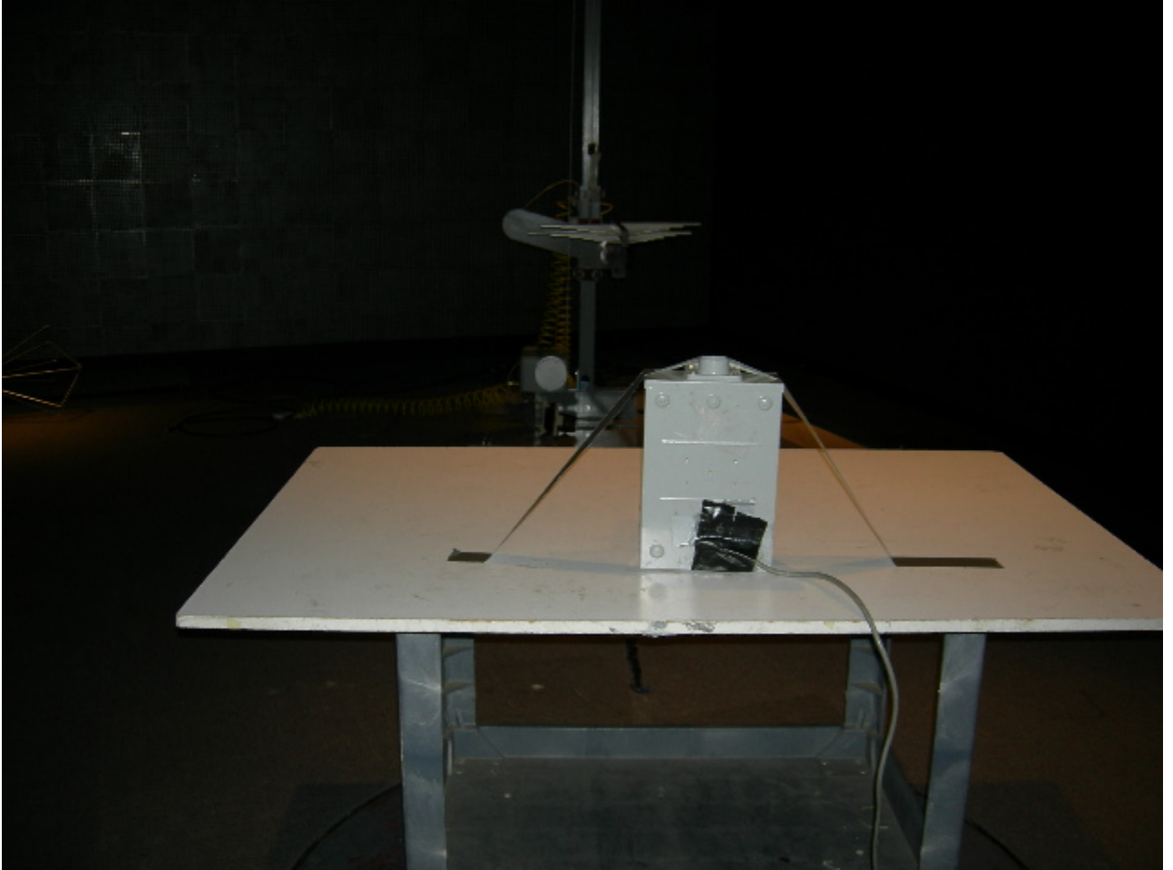
Figure 3: Radiated Emissions – Unintentional
