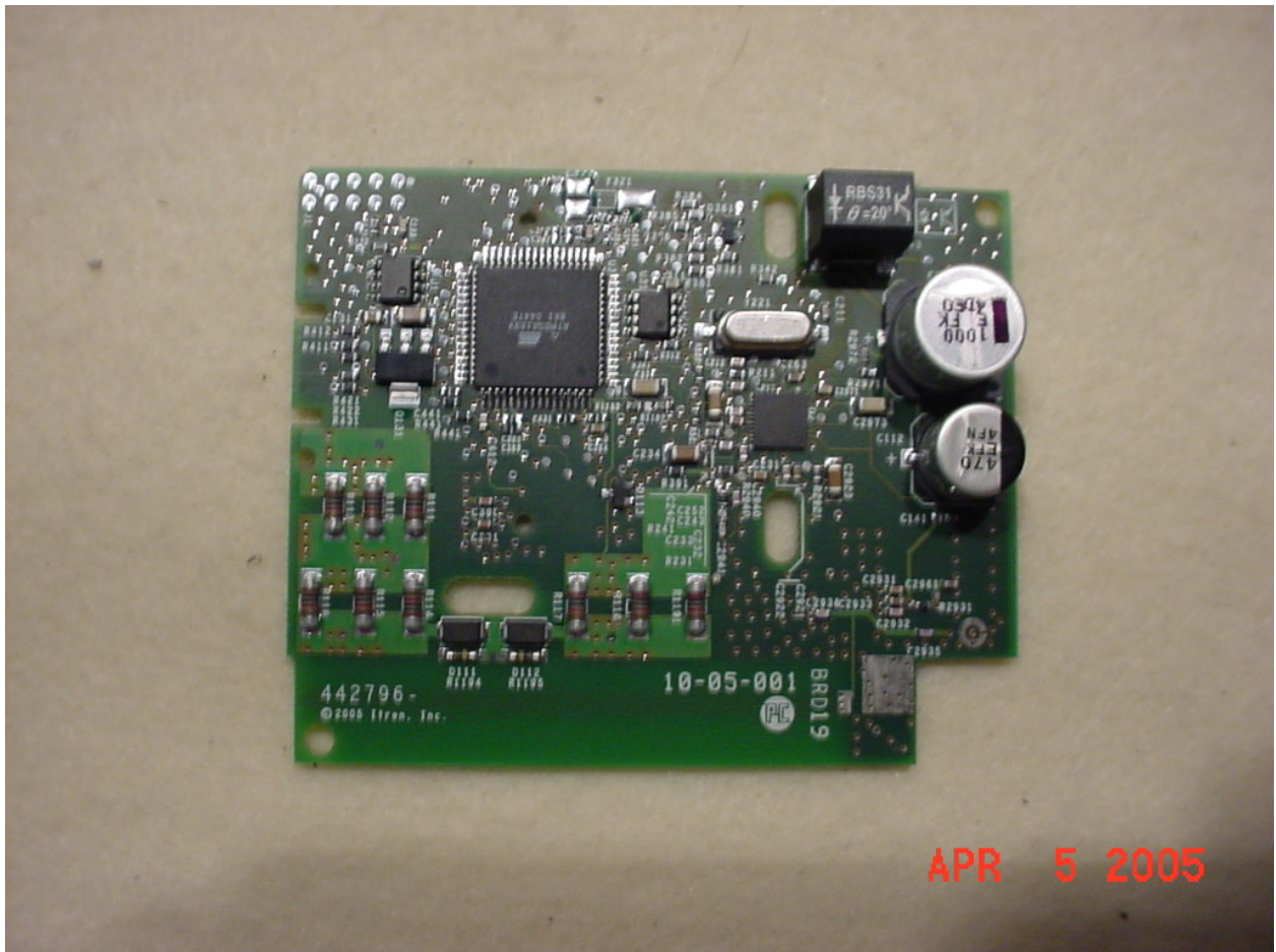
Figure 3: PCB Front View
