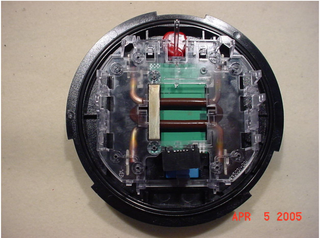
Figure 7: Meter Base Top View
