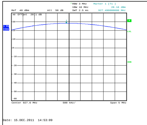
Figure 7.2.2-3: Output Power – HCH – FSK 150kbps
