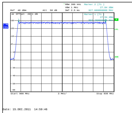
Figure 7.3.2-1: Hopping Channels - FSK Modulation 150kbps
