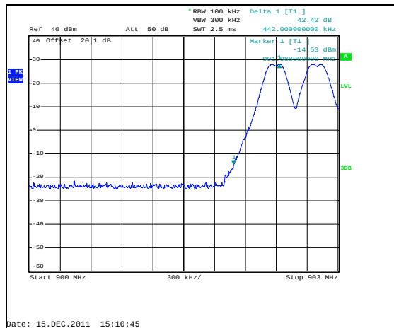
Figure 7.4.1.2-3: Lower Band-edge – FSK 150kbps
