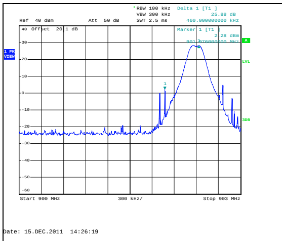
Figure 7.4.1.2-1: Lower Band-edge – FSK 150kbps
