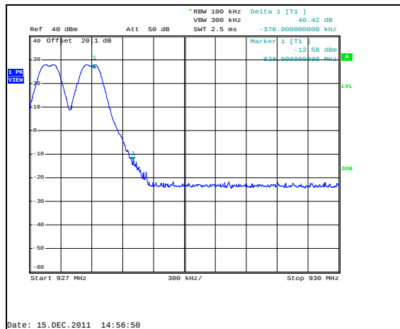
Figure 7.4.1.2-4: Upper Band-edge – FSK 150kbps
