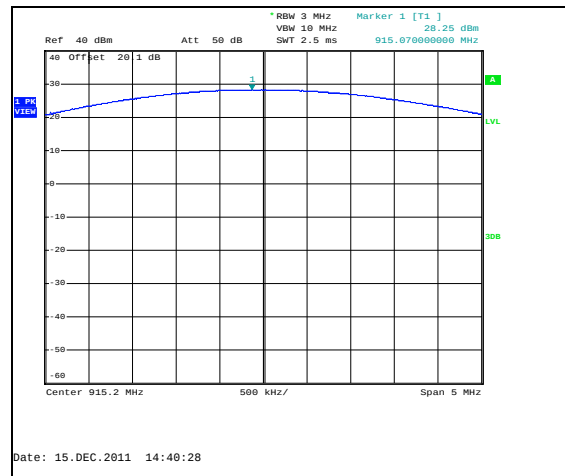
Figure 7.2.2-2: Output Power – MCH – FSK150kbps
