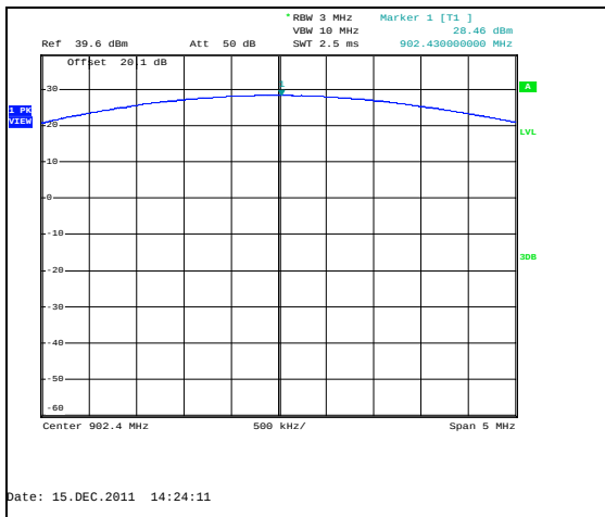
Figure 7.2.2-1: Output Power – LCH – FSK 150kbps
