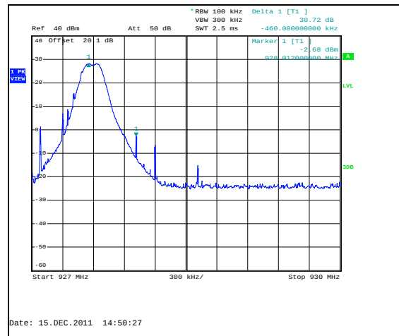
Figure 7.4.1.2-2: Upper Band-edge – FSK 150kbps
