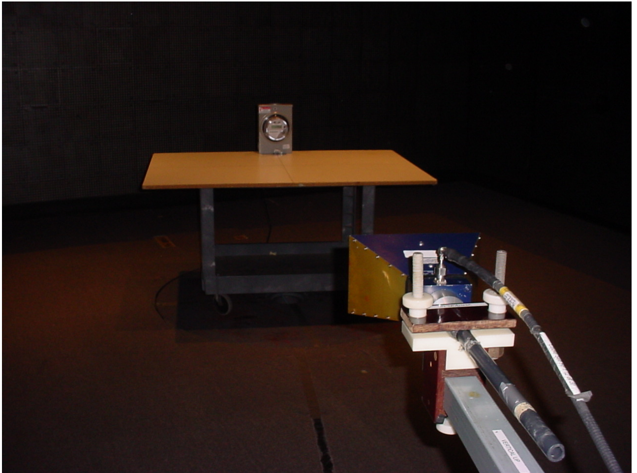
Figure 3: Radiated Emissions – 4S Meter
