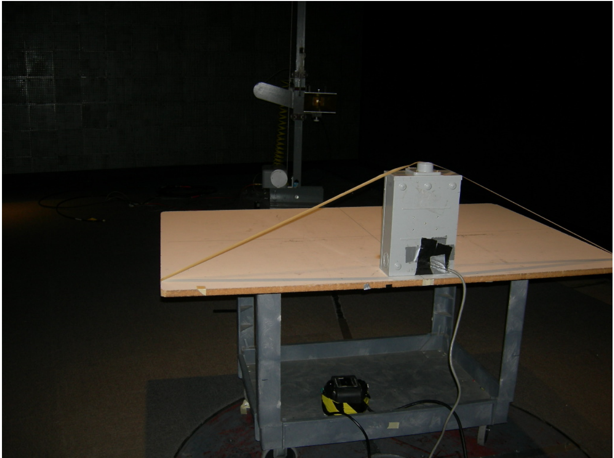
Figure 4: Radiated Emissions – 2S Meter
