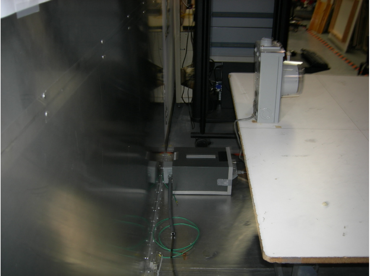
Figure 8: AC Power Line Conducted Emissions – 1S Meter
