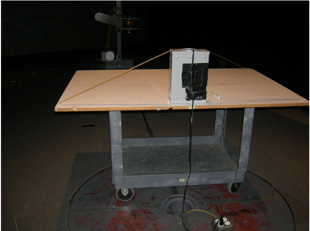
Figure 6: Radiated Emissions – 12S Meter
