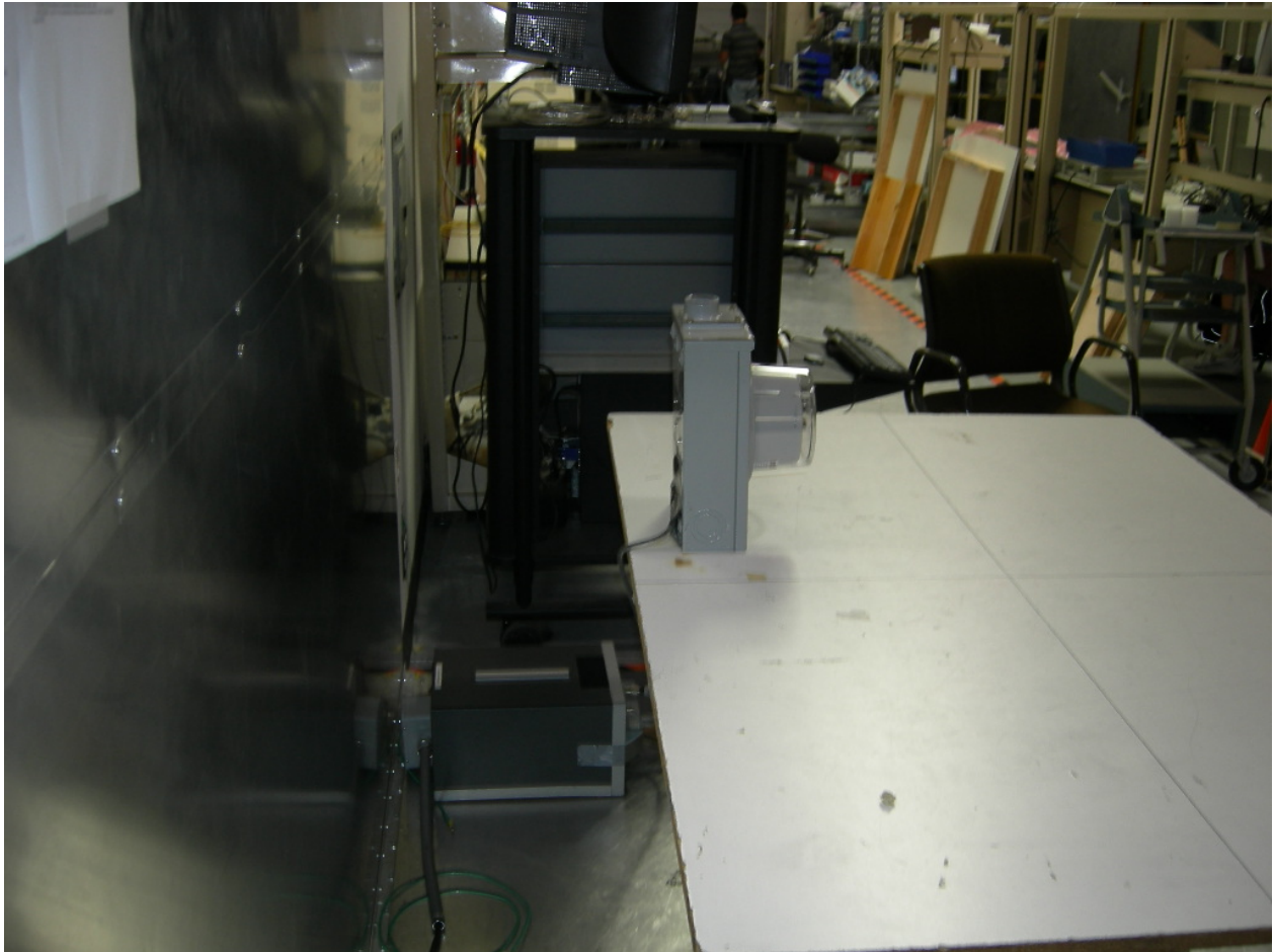
Figure 10: AC Power Line Conducted Emissions – 2S Meter
