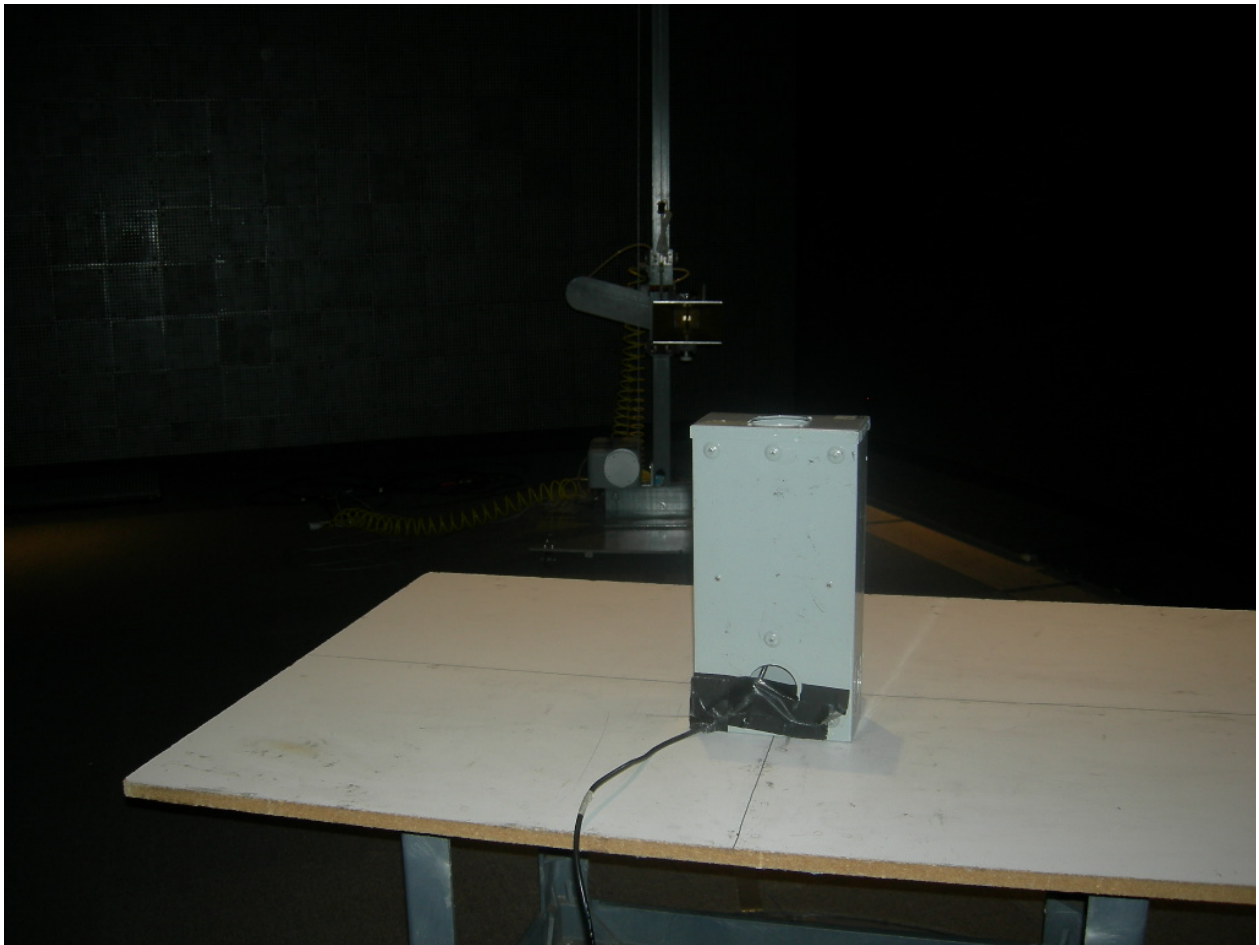
Figure 3: Radiated Emissions – Host 2S Meter Type
