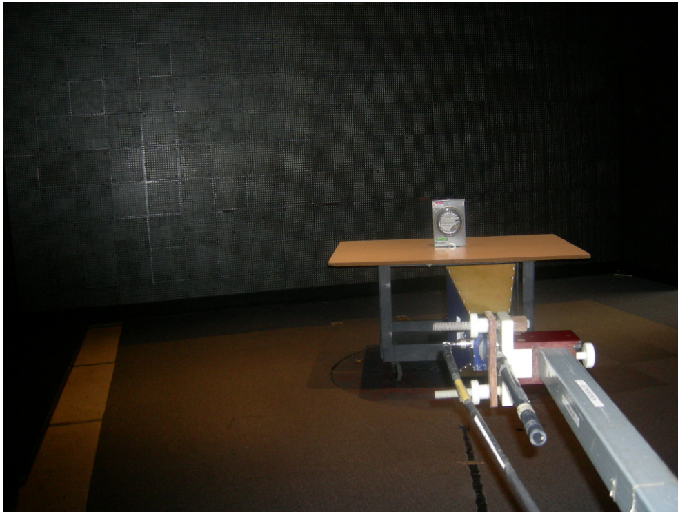
Figure 9: Radiated Emissions – Host 12S Mono Meter Type
