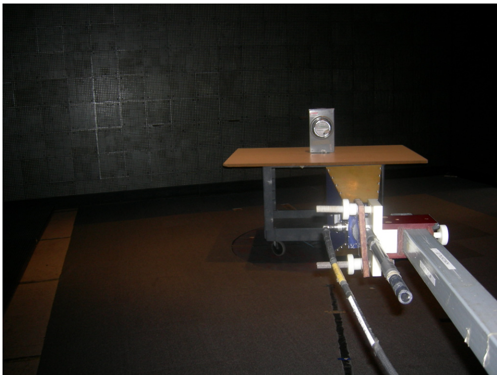
Figure 18: Radiated Emissions – Host 36S Poly Meter Type
