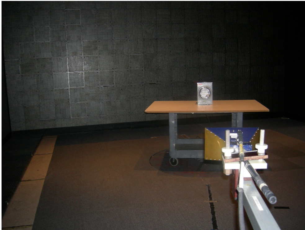
Figure 7: Radiated Emissions – Host 4S Mono Meter Type
