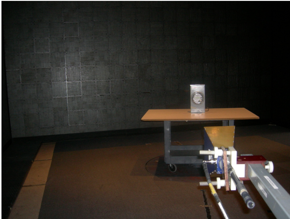
Figure 3: Radiated Emissions – Host 2S Mono Meter Type
