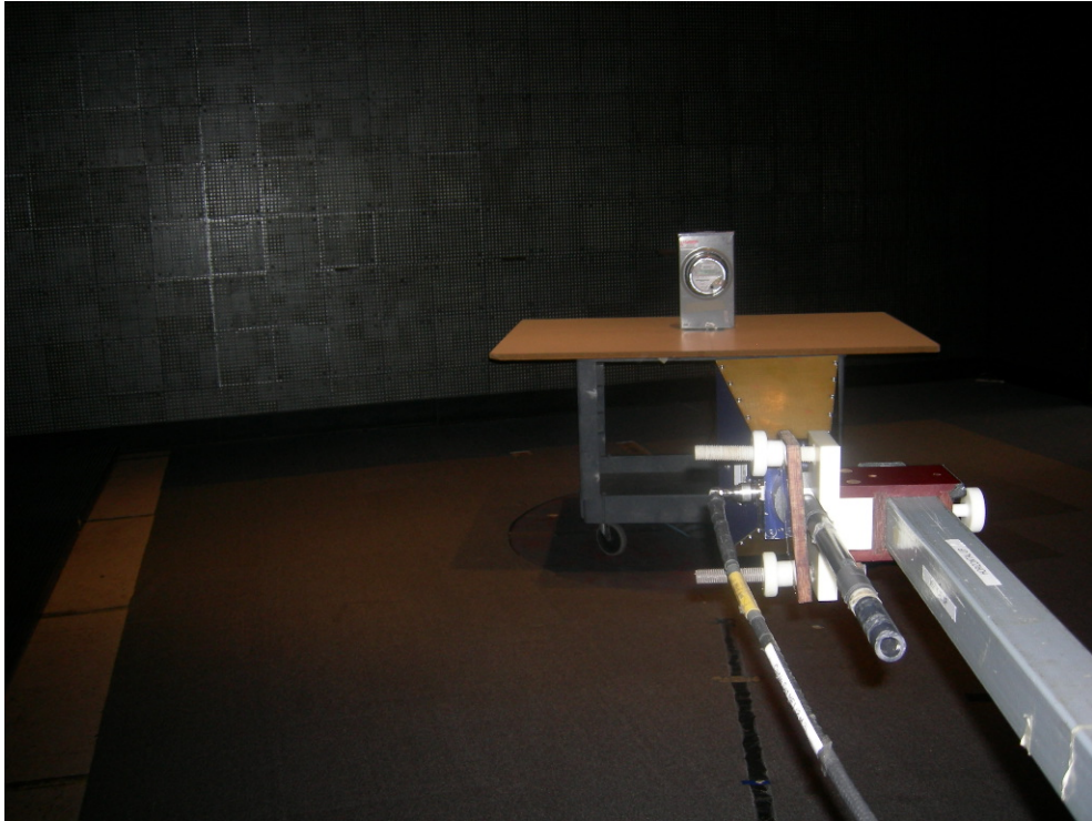
Figure 17: Radiated Emissions – Host 36S Poly Meter Type
