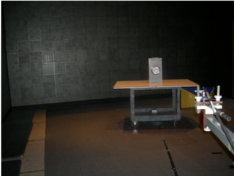
Figure 15: Radiated Emissions – Host 16S Poly Meter Type
