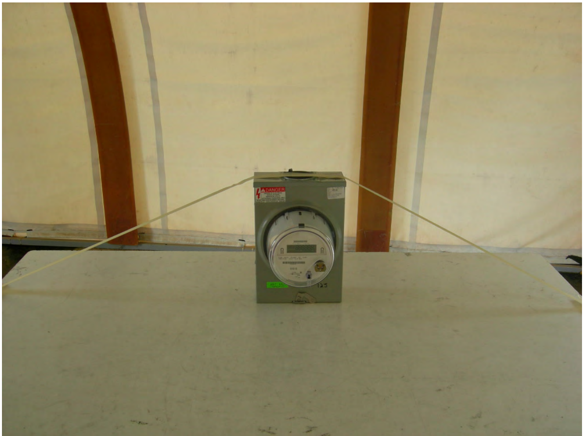
Figure 17: 12S Host – Intentional Radiated Emissions
