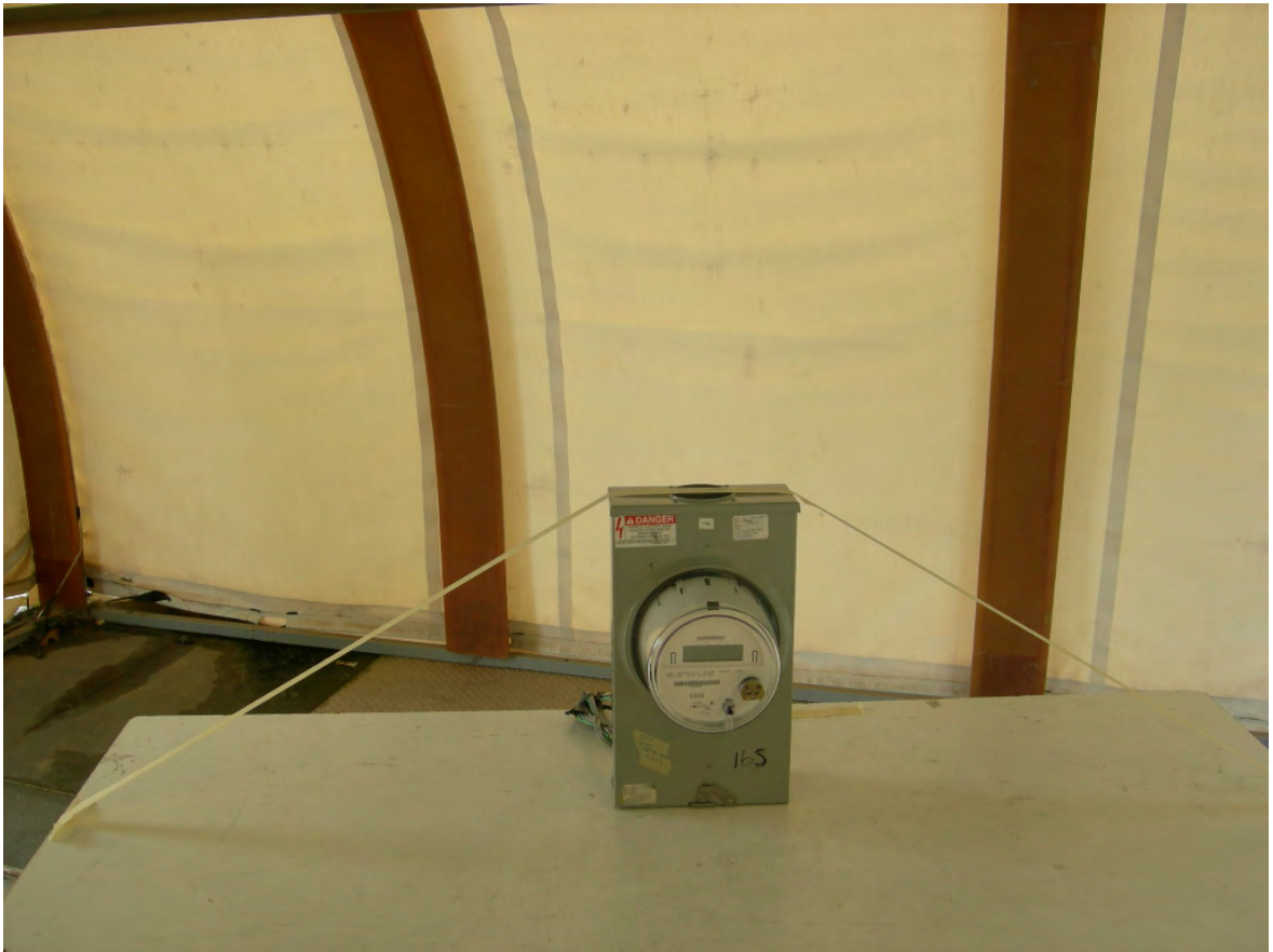
Figure 21: 16S Host – Intentional Radiated Emissions
