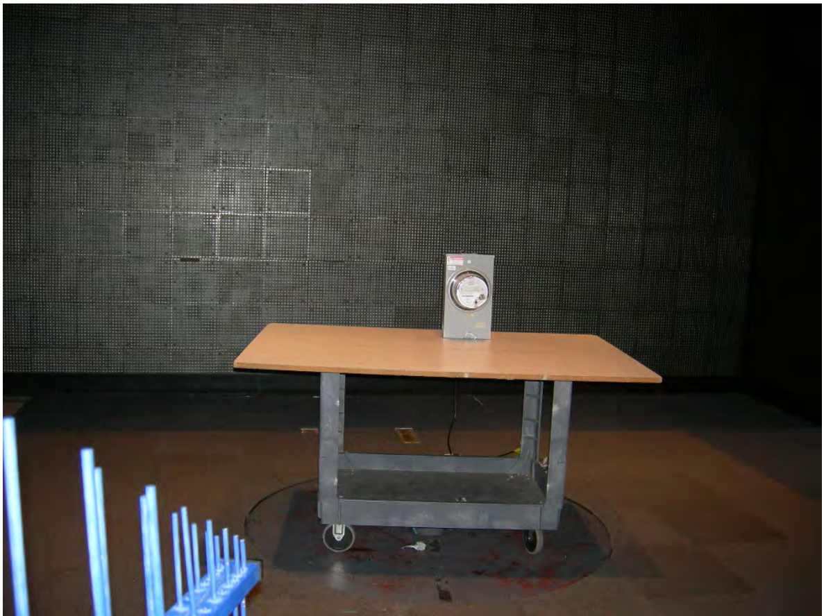
Figure 10: 9S(8S) Host – Unintentional Radiated Emissions
