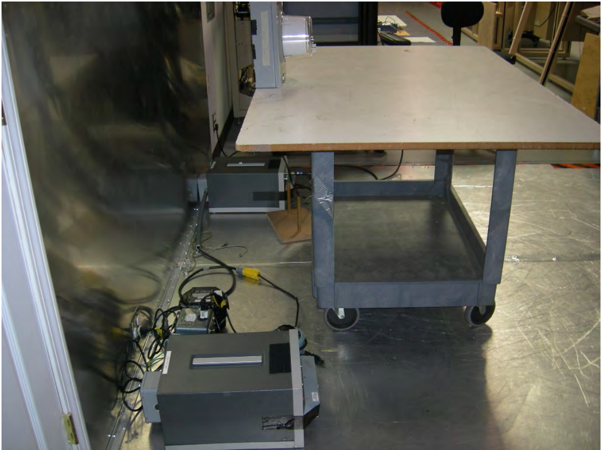
Figure 20: 12S Host – AC Power Line Conducted Emissions
