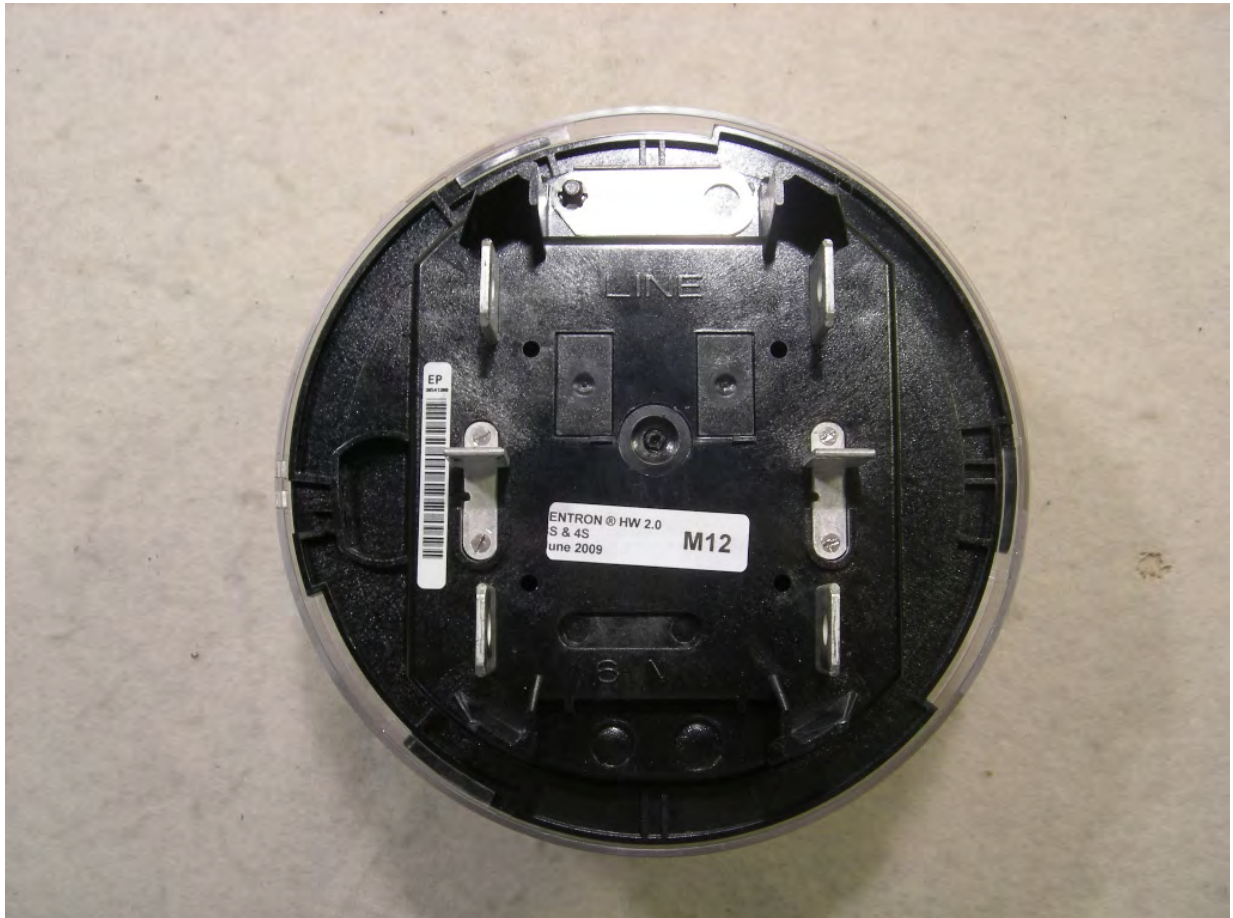
Figure 6: 4S Host
