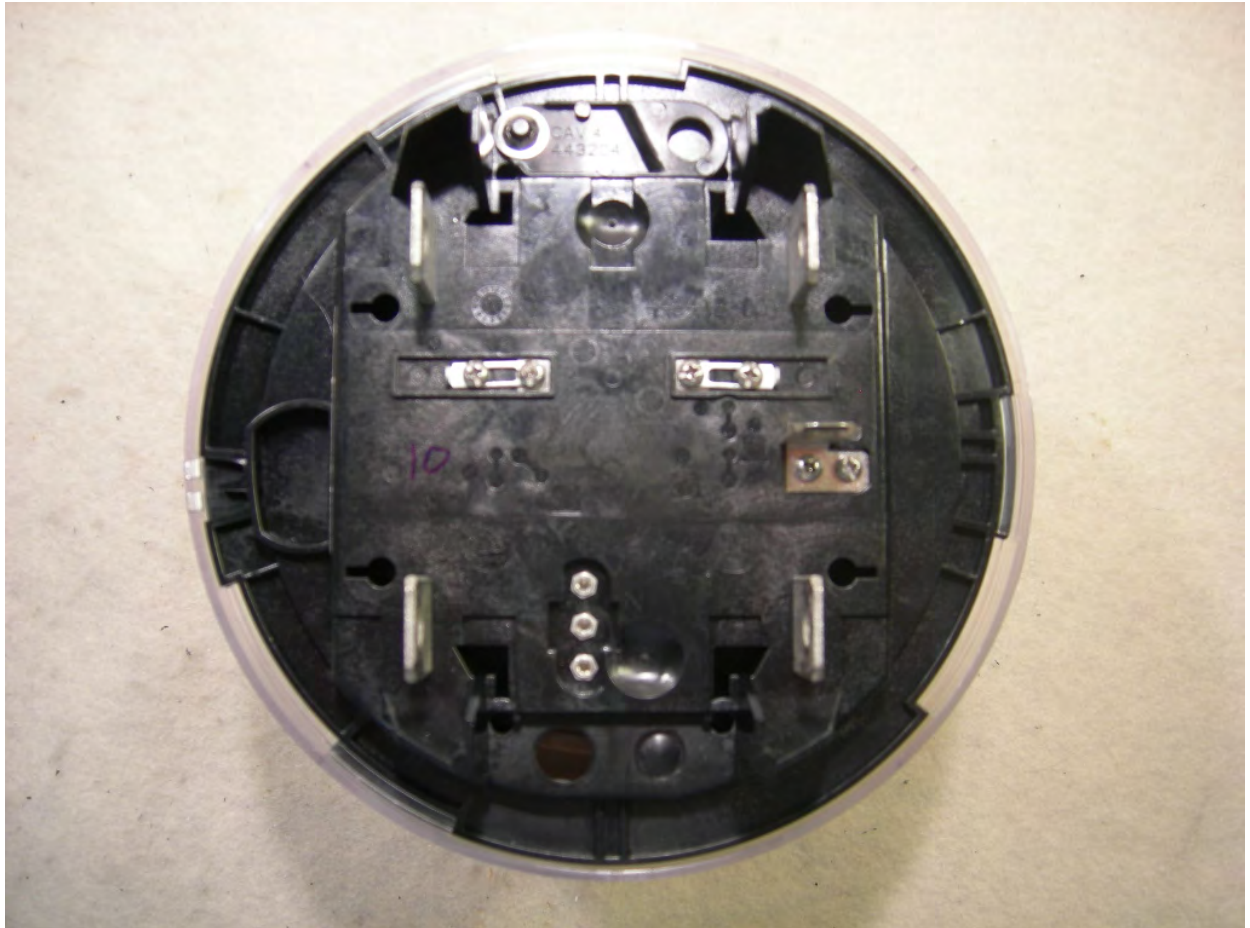
Figure 15: 12S Host
