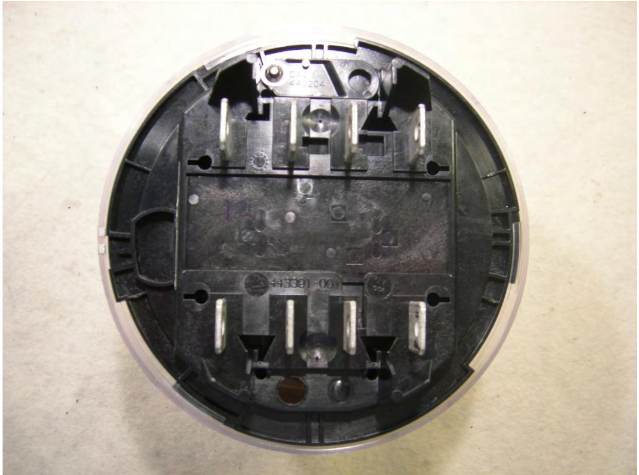
Figure 21: 45S(5S) Host
