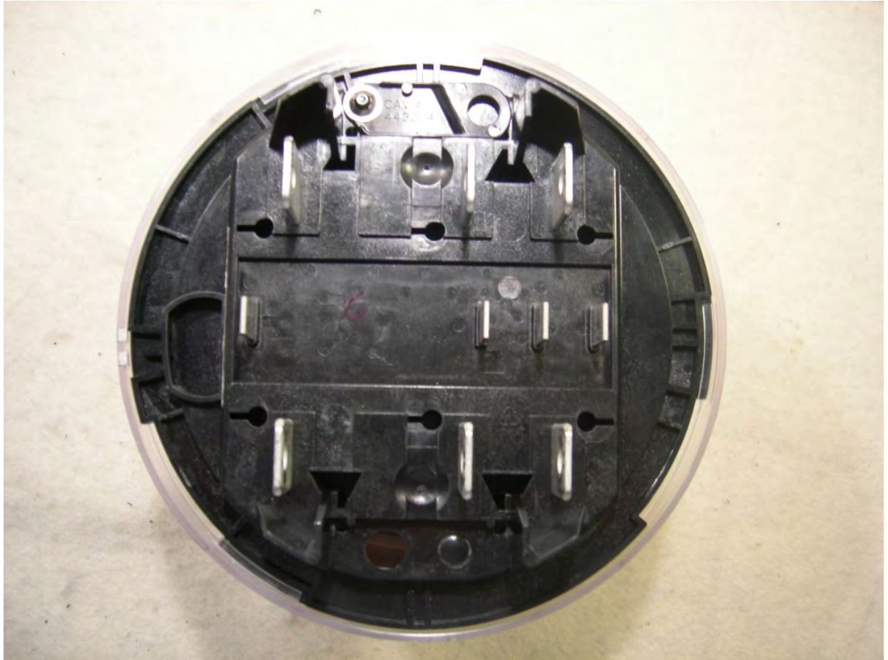
Figure 9: 9S(8S) Host
