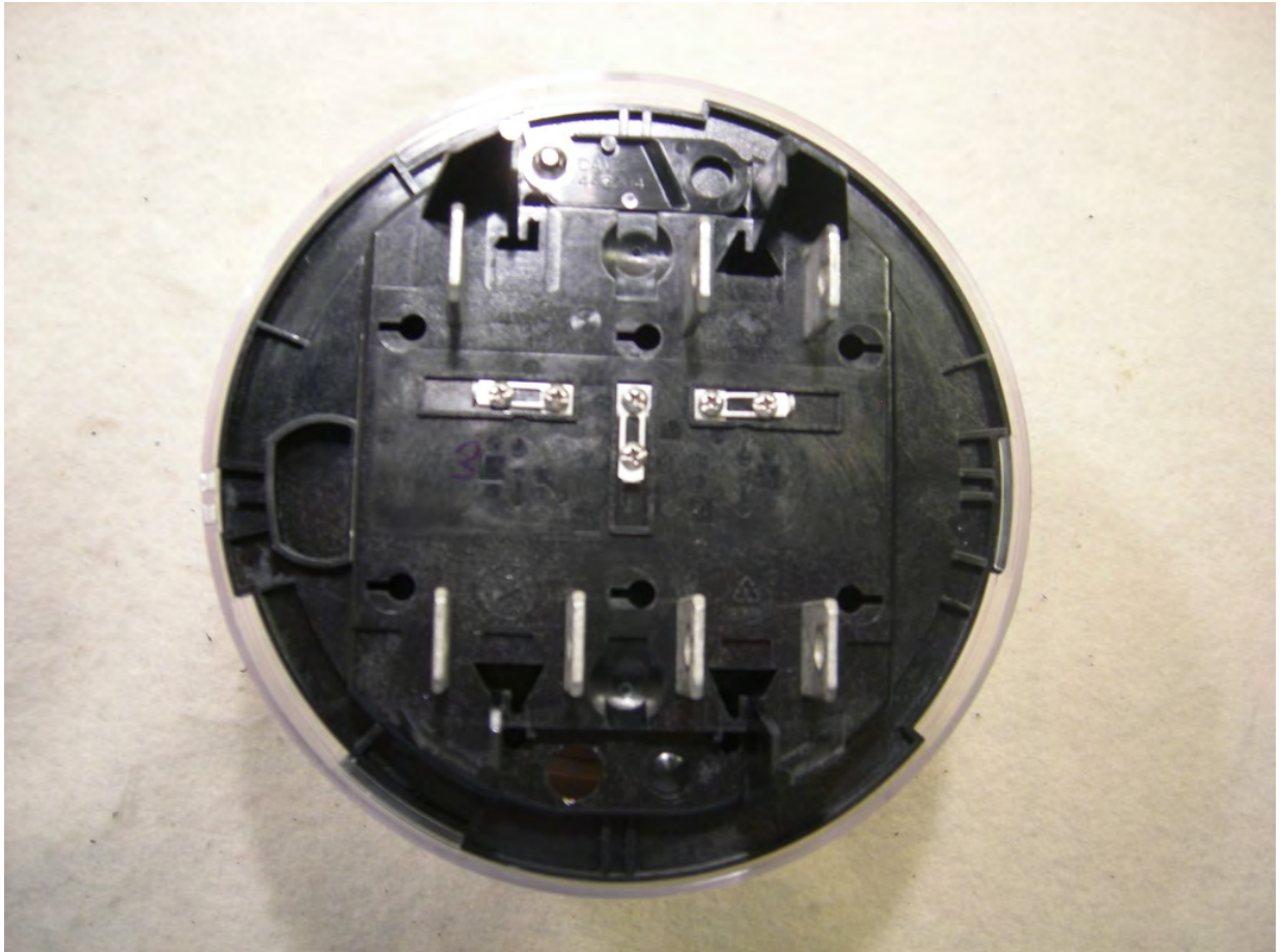
Figure 18: 16S Host
