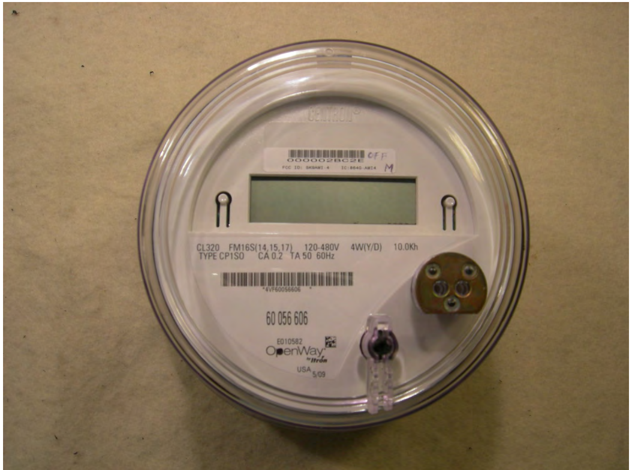
Figure 16: 16S Host
