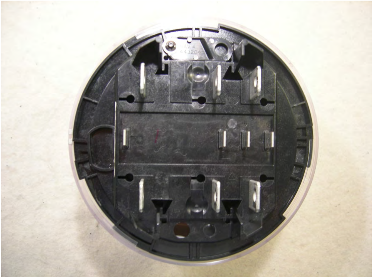
Figure 12: 9/36S Host
