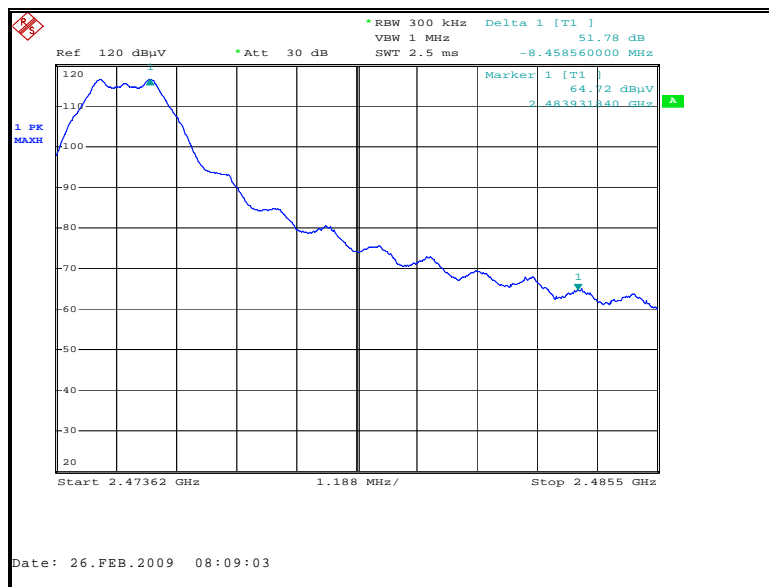
Figure 7.6.1.2-2: Upper Band-edge (Radiated) – 2S
