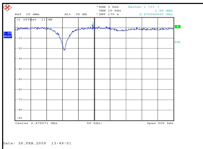
Figure 7.7.2-3: Power Spectral Density Plot – High Channel
