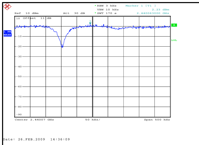
Figure 7.7.2-2: Power Spectral Density Plot – Mid Channel
