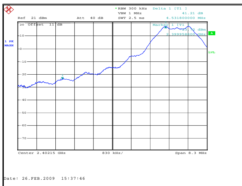
Figure 7.6.1.2-4: Lower Band-edge (Conducted)
