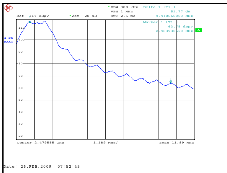
Figure 7.6.1.2-3: Upper Band-edge (Radiated) – 12S
