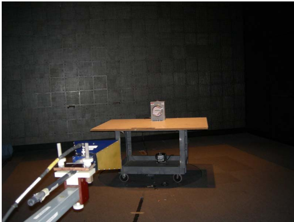
Figure 1: Radiated Emissions – Host 2S Meter Type
