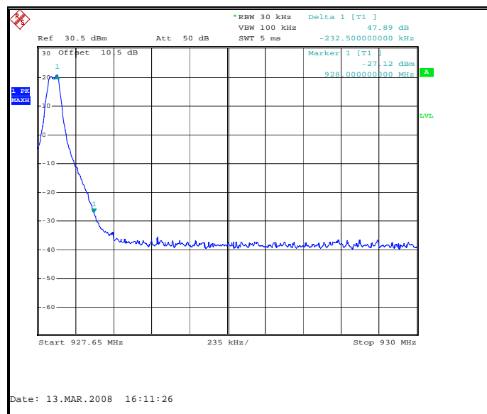
Figure 7.6.1-2: Upper Band-edge
