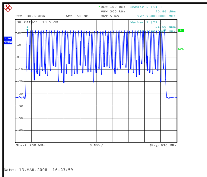
Figure 7.5.2-1: Number of Hopping Channels
