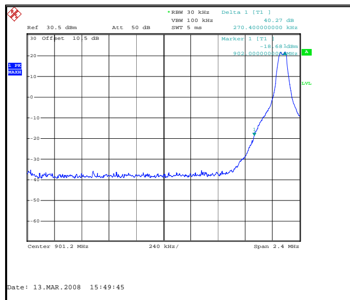
Figure 7.6.1-1: Lower Band-edge
