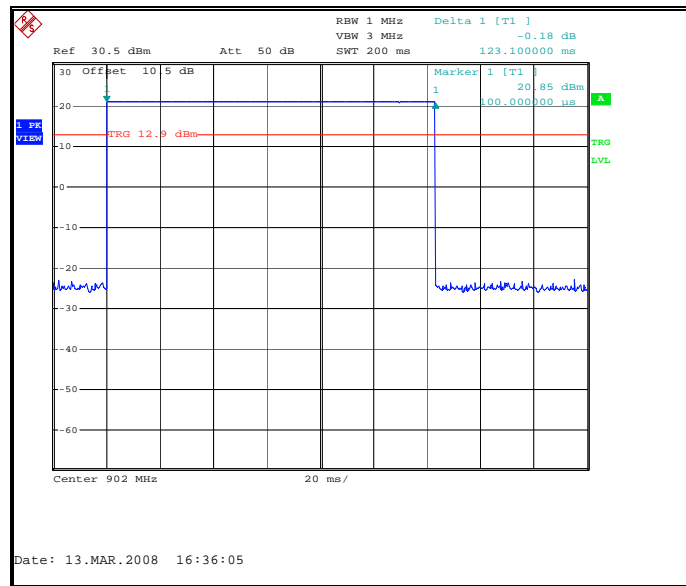
Figure 7.5.3-1: Channel Dwell Time
