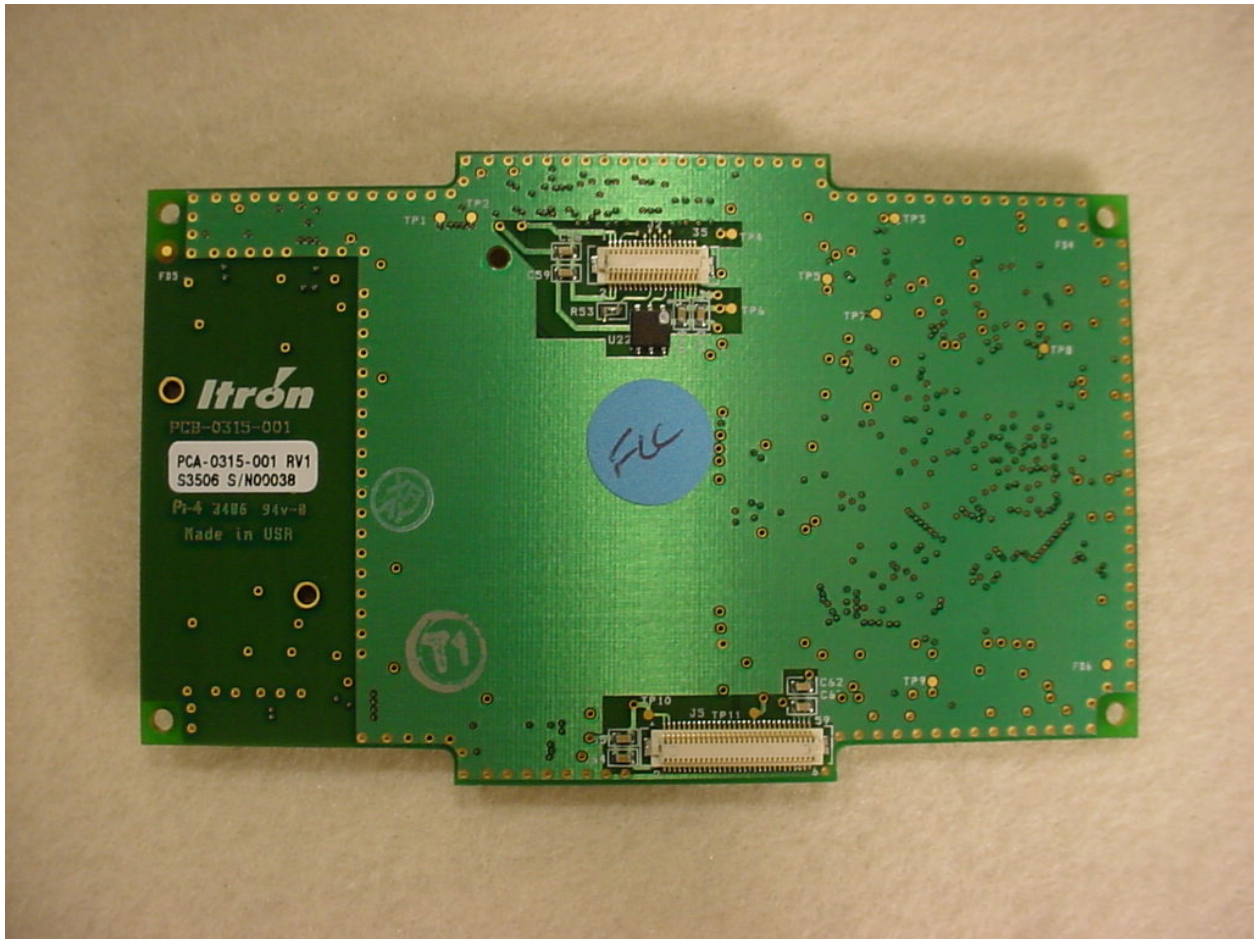
Figure 9: Internal – Mezzanine GPRS Modem Board Back
