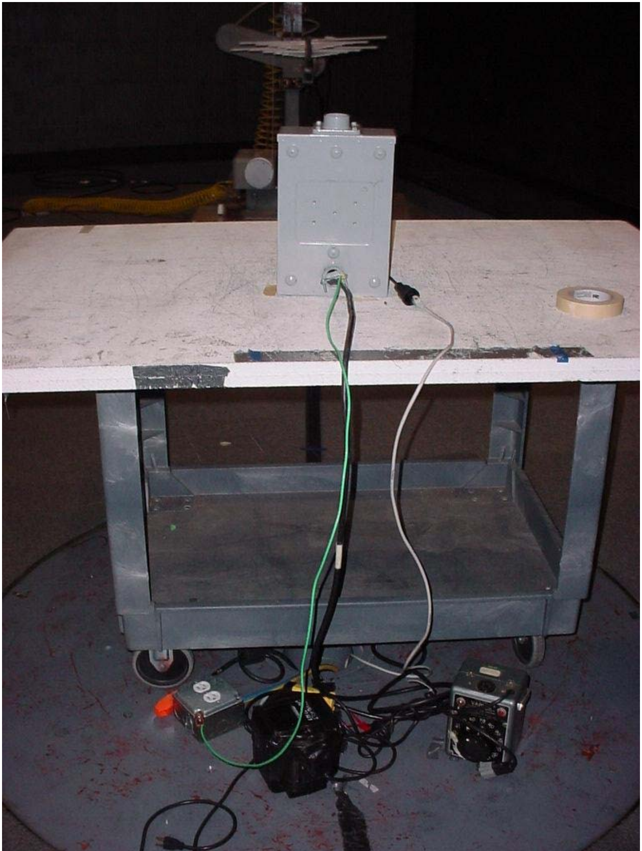
Figure 12: Test Setup – Radiated Emissions - Unintentional
