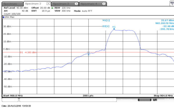
Figure 7.6.1.2-5: Lower Band-edge – No Hopping
