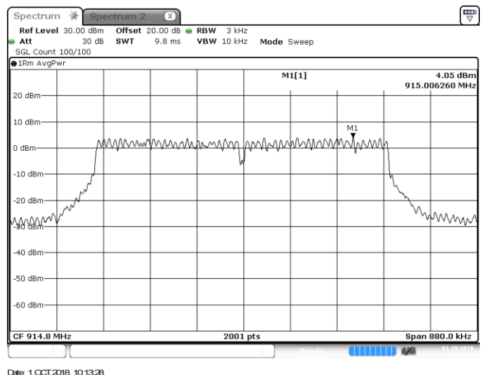
Figure 7.7.2-2: Power Spectral Density – MCH
