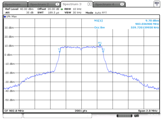
Figure 7.3.2-4: 99% Occupied Bandwidth – LCH
