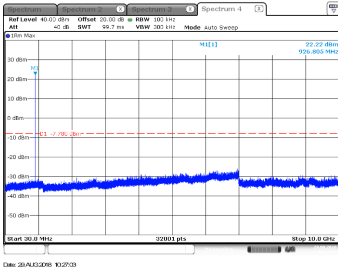
Figure 7.6.1.2-3: 30 MHz – 10 GHz –High Channel
