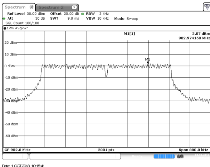
Figure 7.7.2-1: Power Spectral Density – LCH
