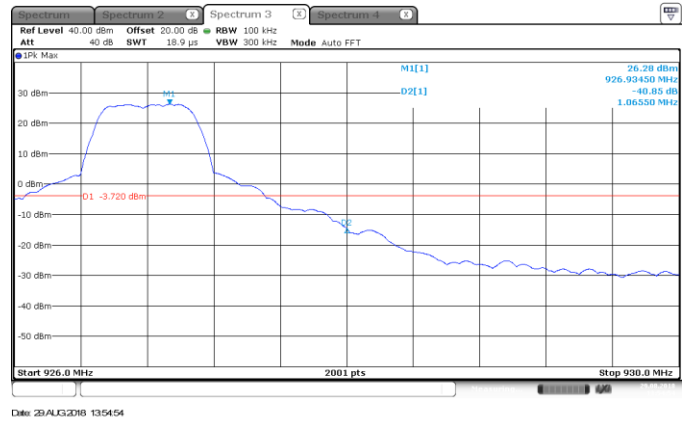
Figure 7.6.1.2-6: Upper Band-edge - No Hopping
