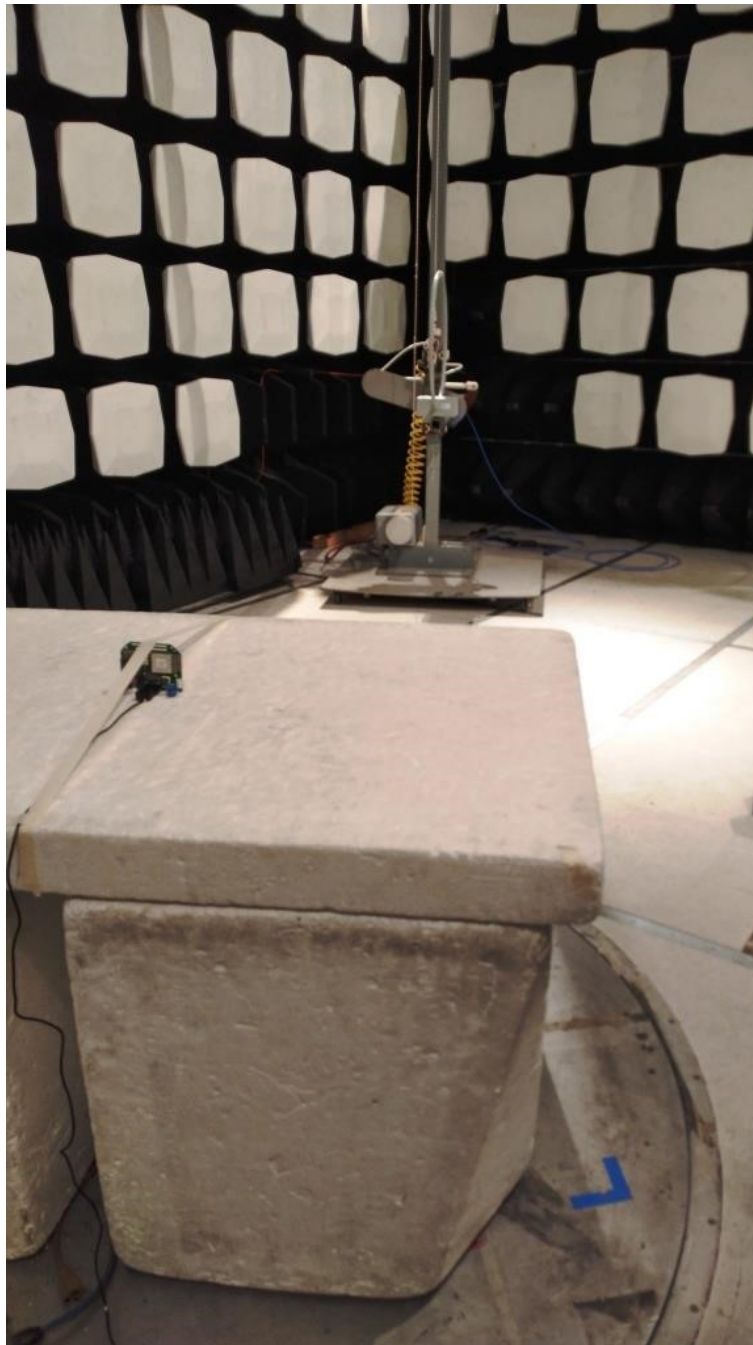
Figure 2: Equipment Under Test – Radiated Emissions – Below 30MHz
