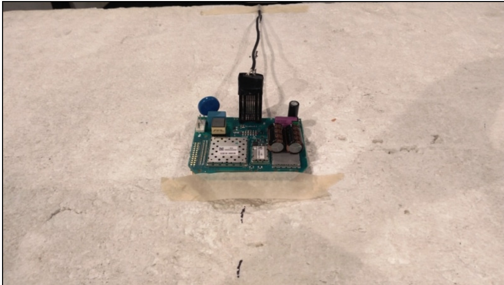
Figure 5: Equipment Under Test – Radiated Emissions – Z-orientation
