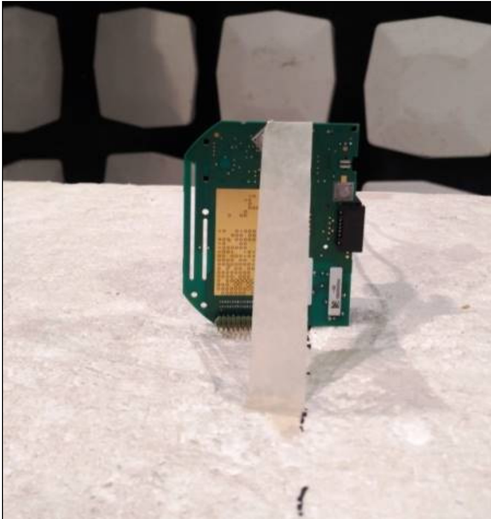
Figure 3: Equipment Under Test – Radiated Emissions – X-orientation
