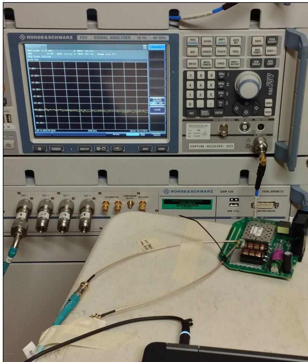
Figure 7: Equipment Under Test – RF Conducted Emissions
