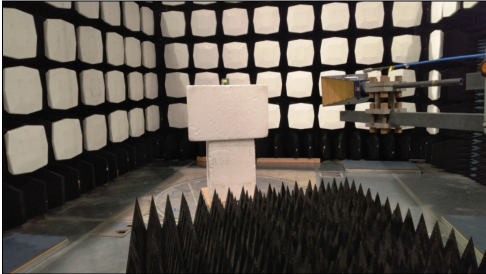
Figure 1: Test Setup – Radiated Emissions – Front View
