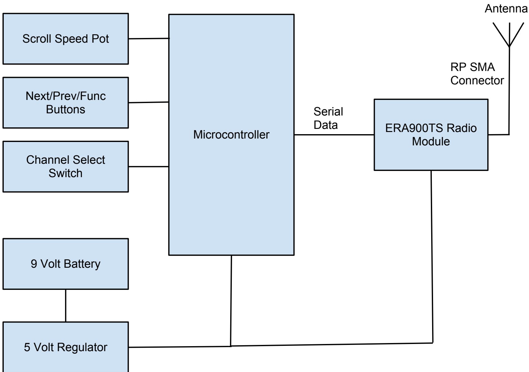
Autoscript Ltd WSC-RAT-A Block Diagram
