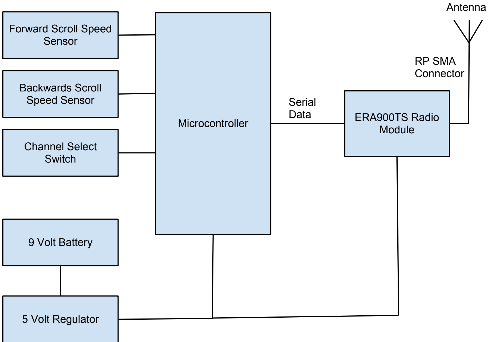
Autoscript Ltd MFC-W-A Block Diagram
