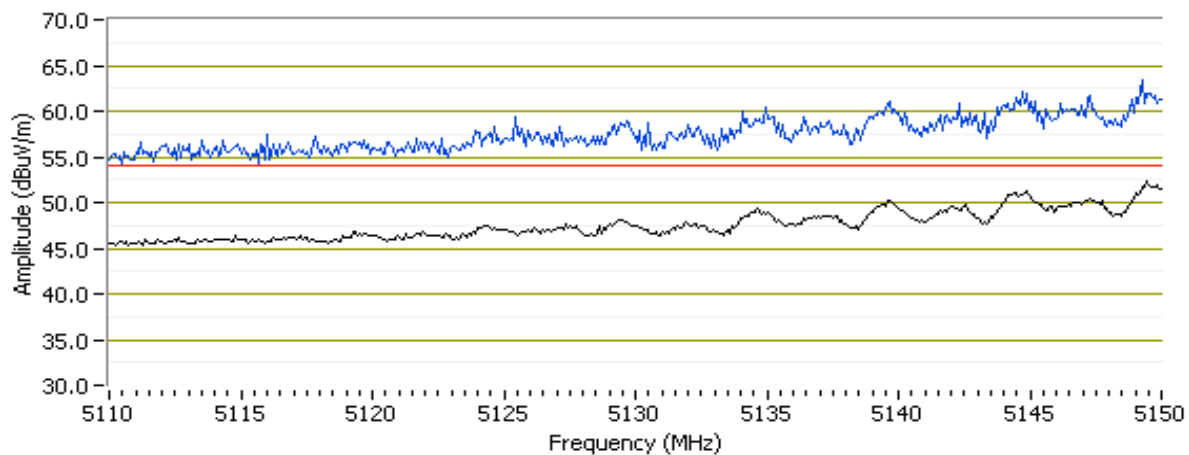
RB 1 MHz; VB 3 kHz (Average) ; RB 1MHz, VB 3MHz Peak (Blue trace)
