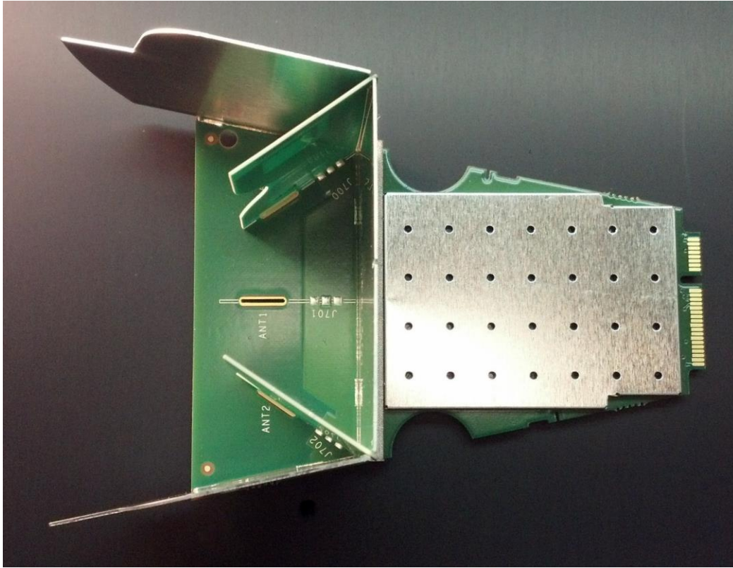
1. Top view
