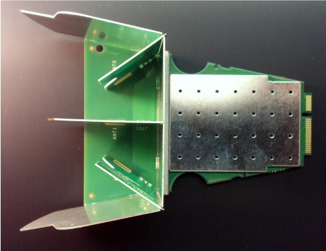
1. Top view
