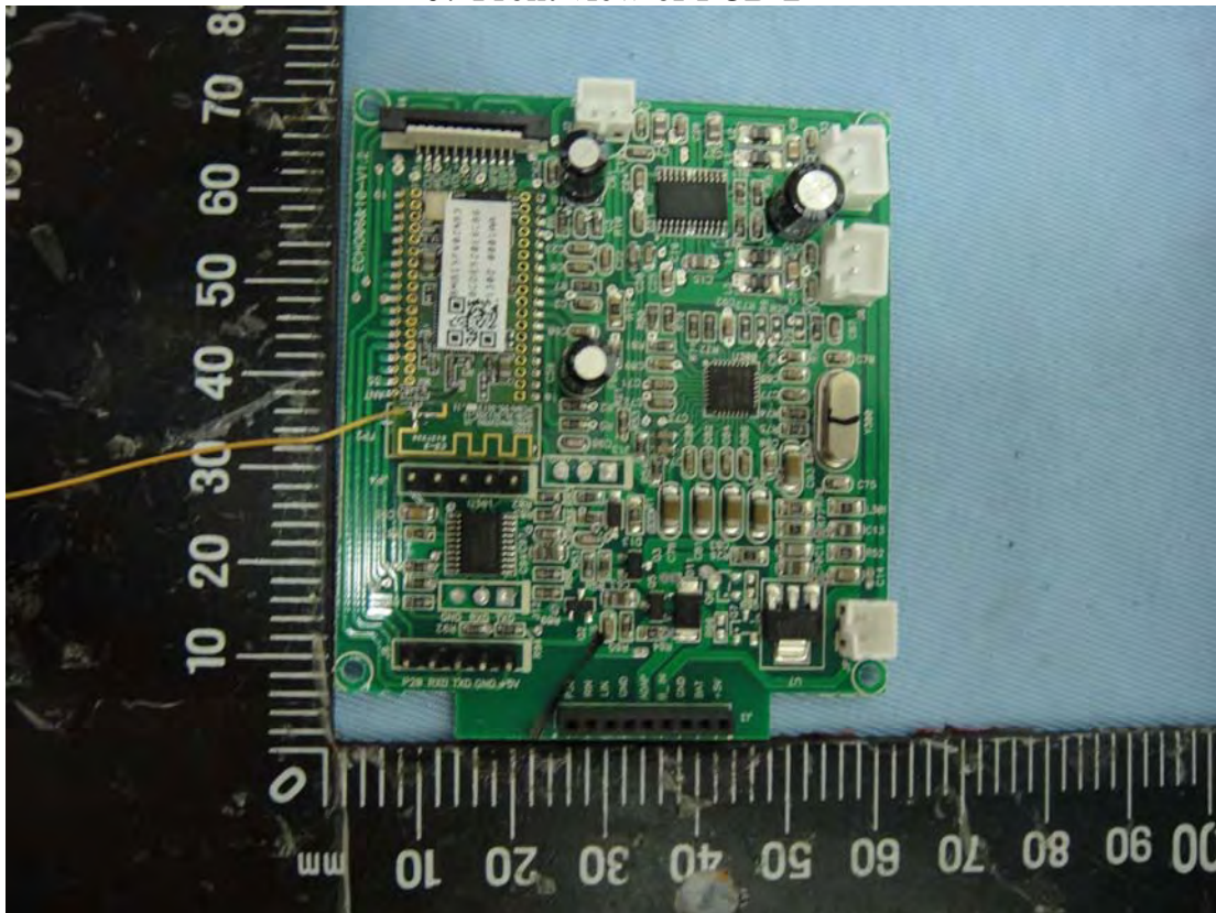
07 Front view of PCB-2
