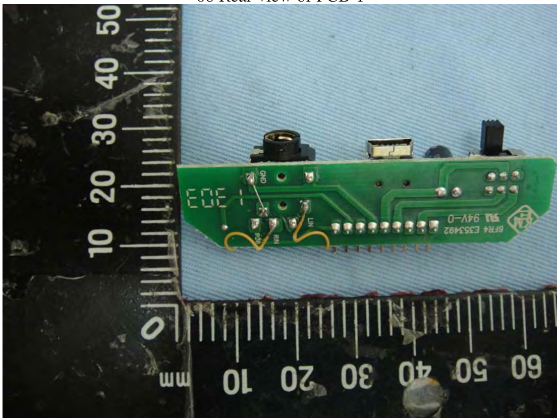
06 Rear view of PCB-1
