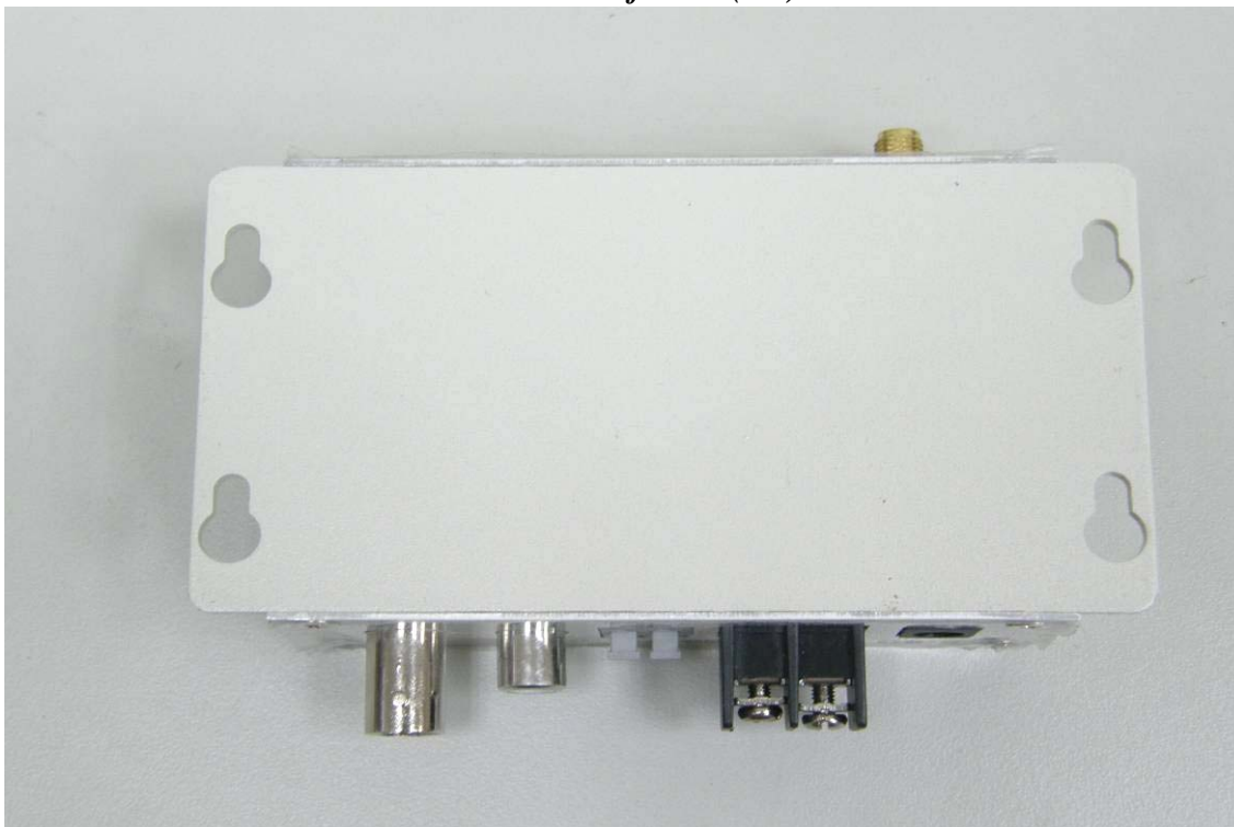
Back View of EUT (TX)
