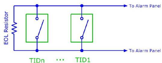
Figure 9 - Normally Open configuration
