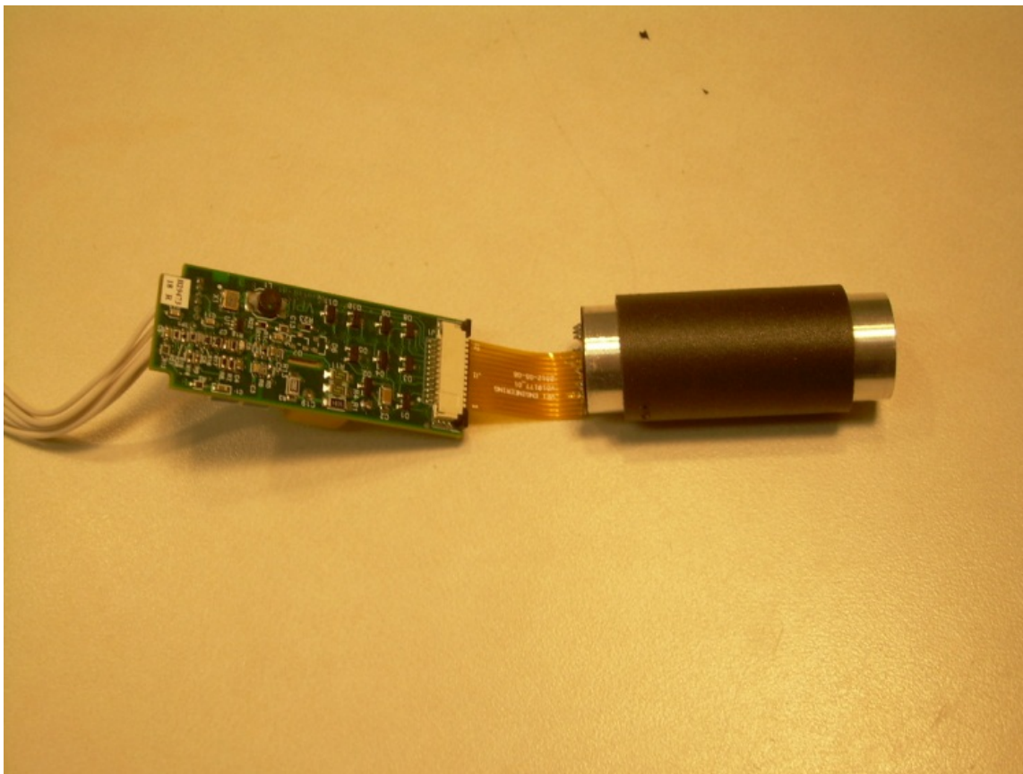
View of the Scintillation Tube and Trace Side of the PCB
