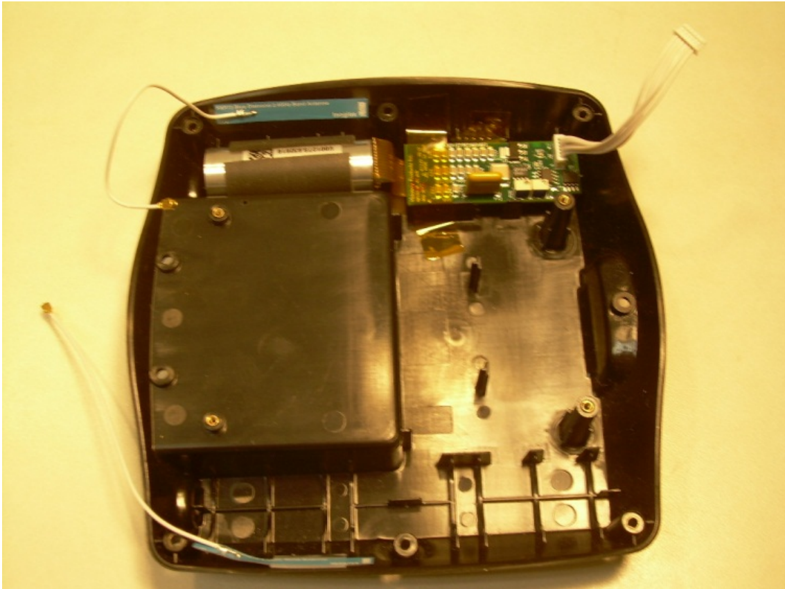
View of the Plastic Housing Showing Antennas, Scintillation Tube, and PCB Placement
