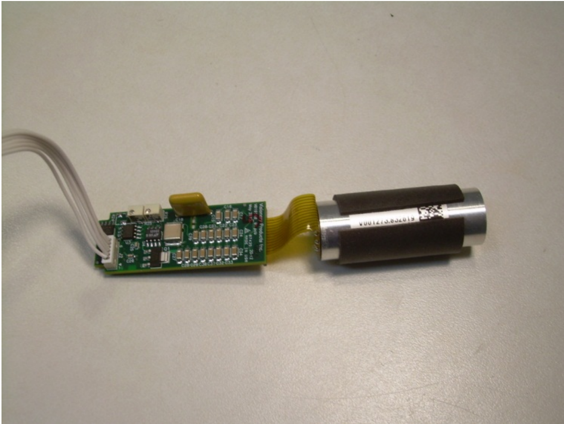
View of the Scintillation Tube and Component Side of the PCB
