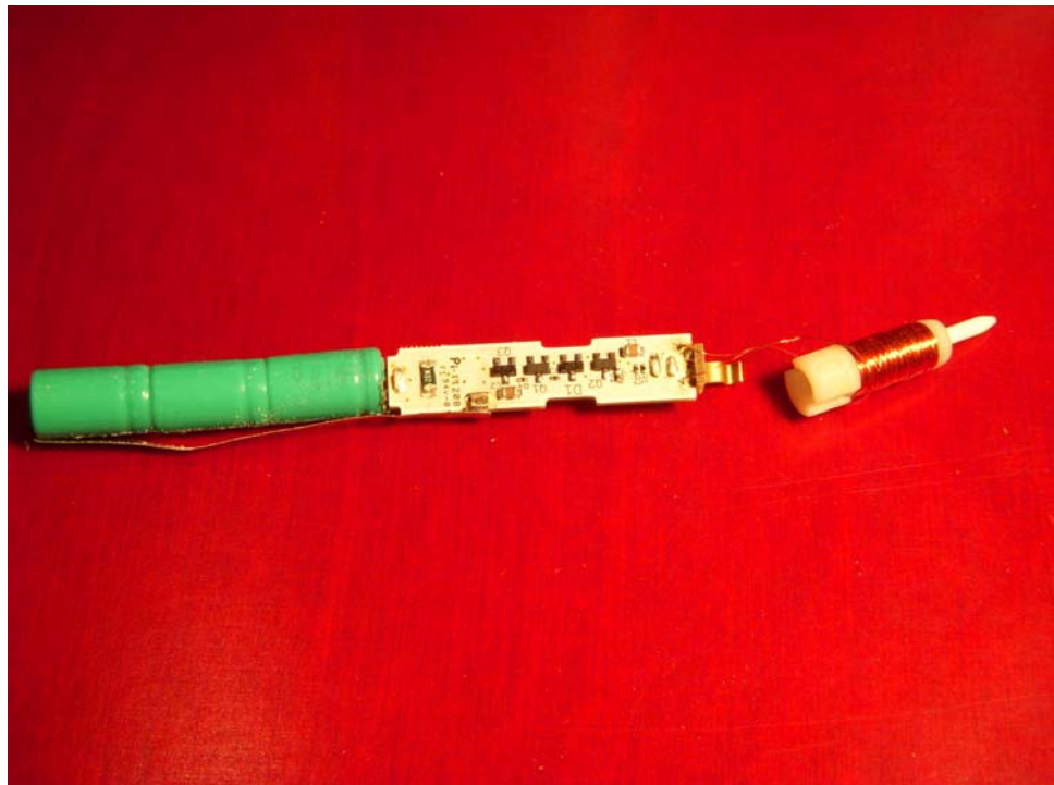
Fig 6 – Q Pen with PCB side 2 shown.
