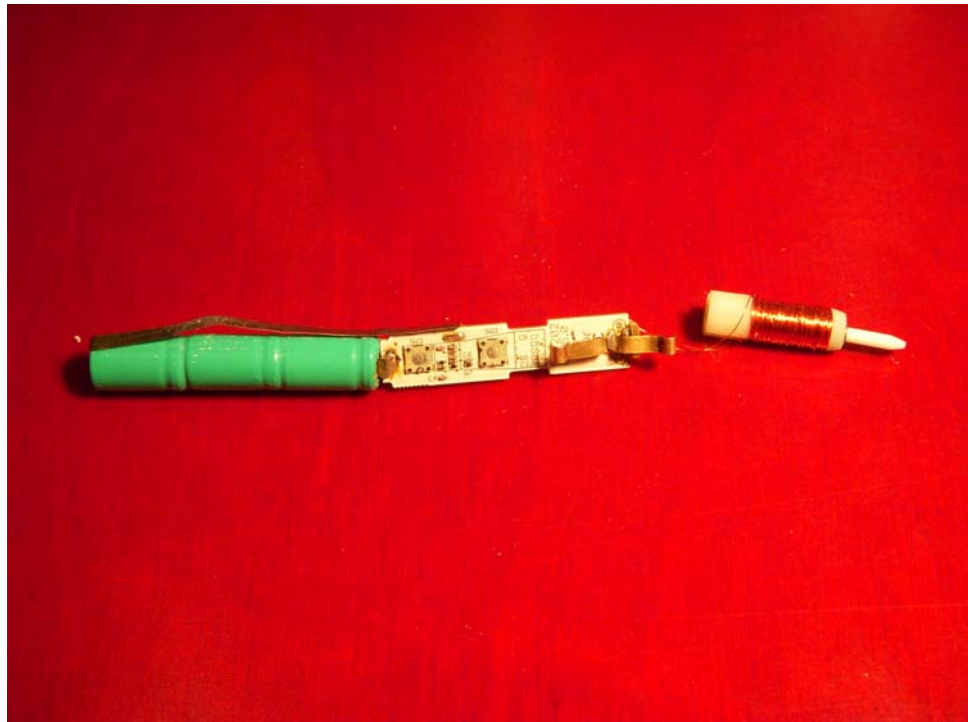
Fig 4 – Q Pen with PCB side 1 shown.
