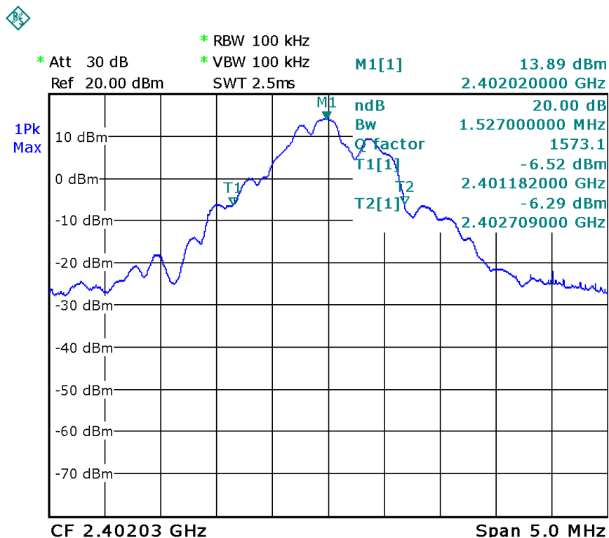
Low Channel
