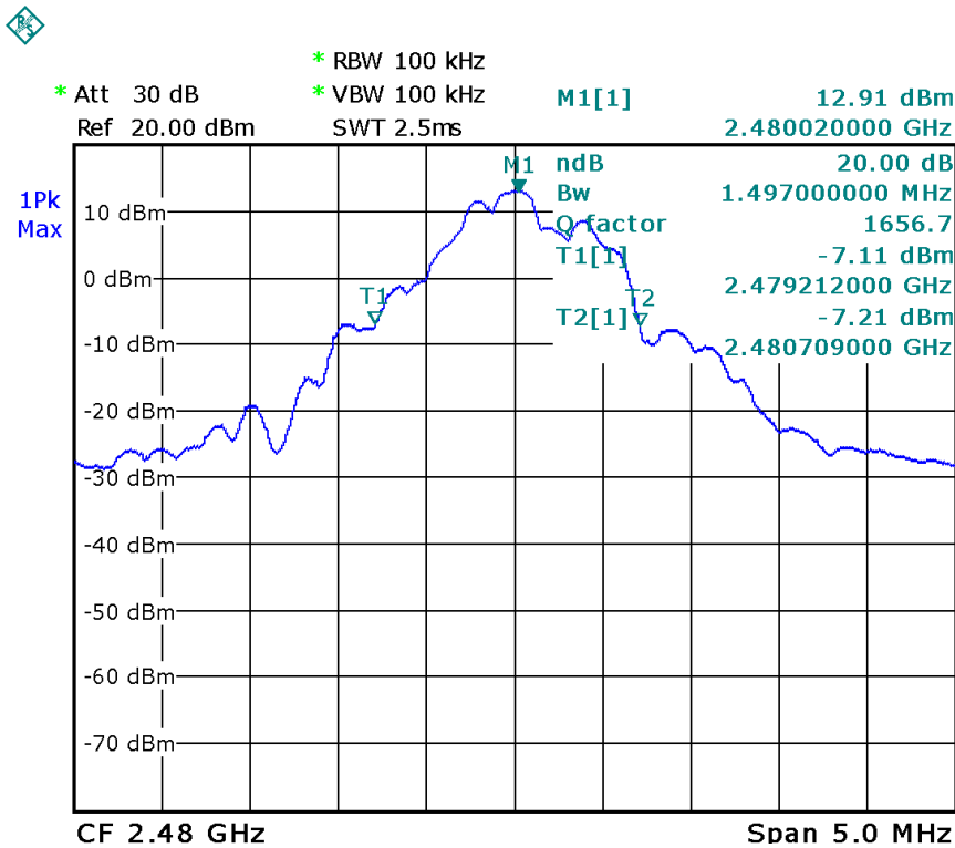
High Channel
