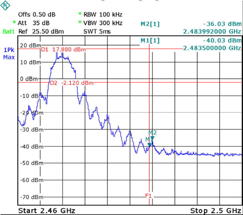
Transmitting Band edge-right side
