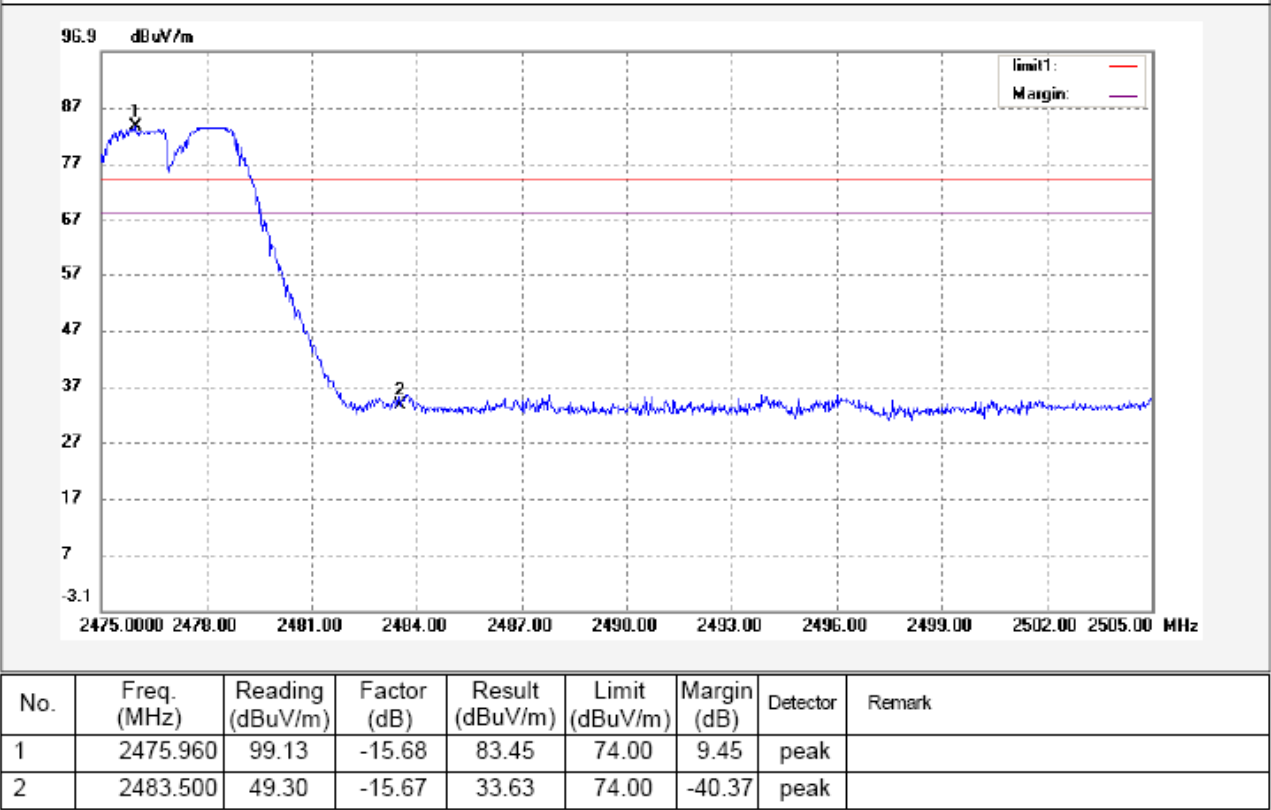
Upper Channel (Hopping on)–Horizontal
