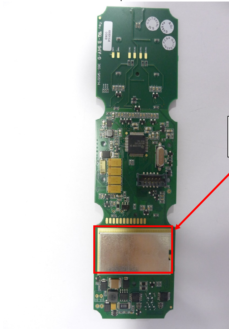
Mainboard – Top View with Shield
