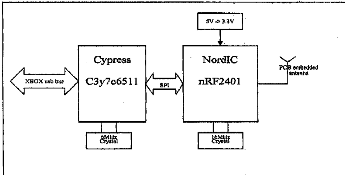
Receiver Block Diagram
