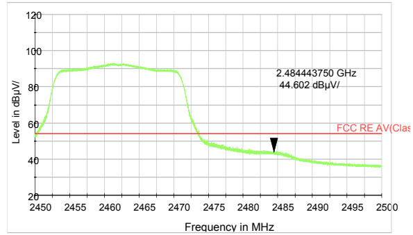
802.11n HT20 -Channel 11 Average
