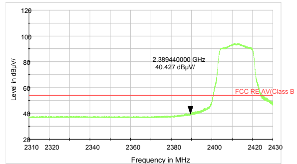
802.11g-Channel 1 Average
