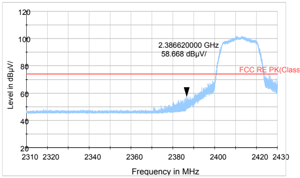
802.11n HT20 -Channel 1 Peak
