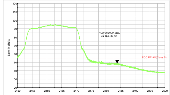
802.11g-Channel 11 Average
