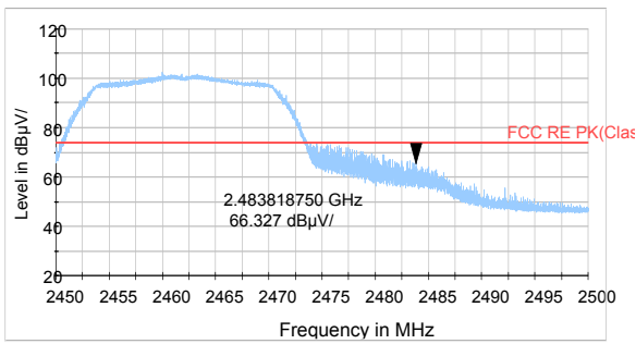
802.11n HT20 -Channel 11 Peak
