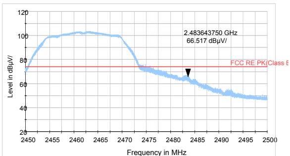
802.11g-Channel 11 Peak
