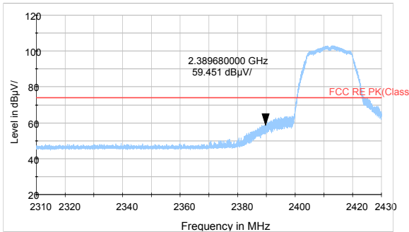
802.11g-Channel 1 Peak
