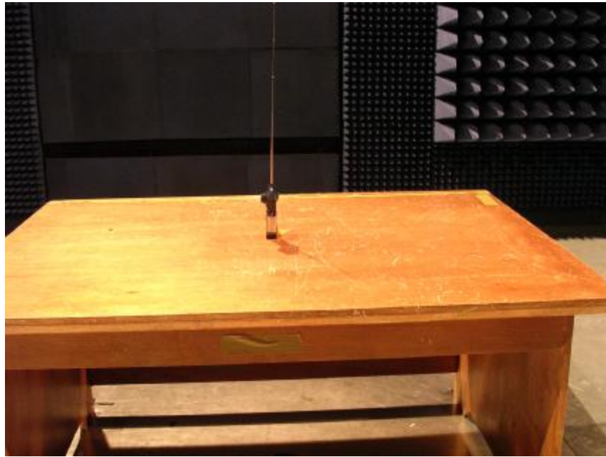
Photo 4: Radiated Emission Test Set-up (Base)
