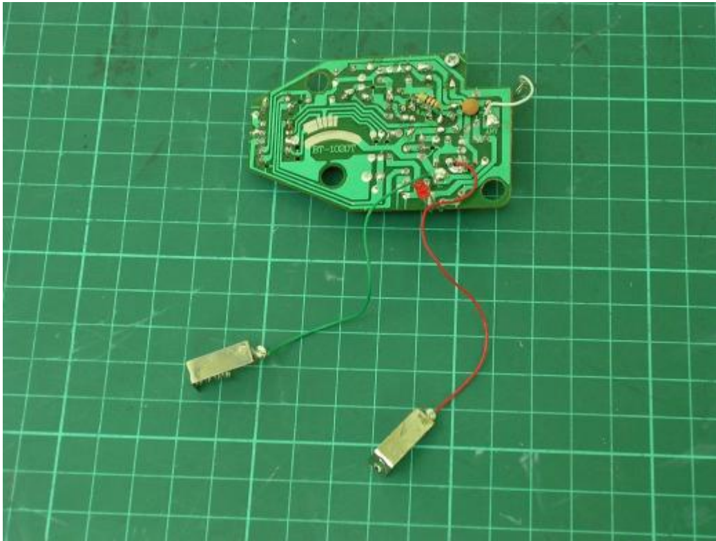
Photo 3: Interior photo of EUT (Remote control)
