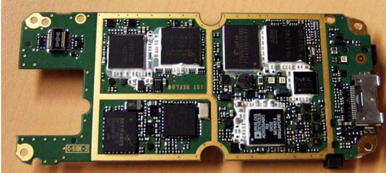
FCC ID SIJVG08 PCB FRONT VIEW
