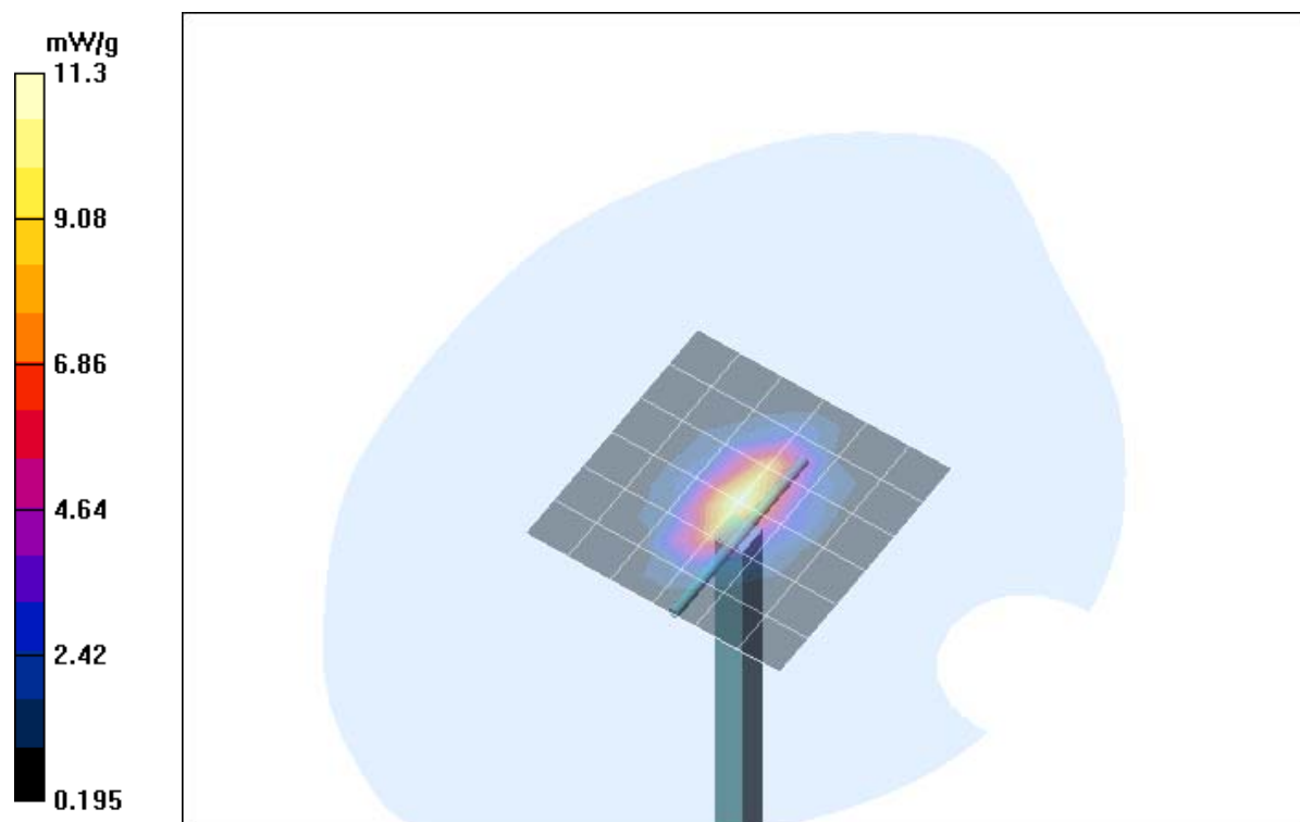
Fig. 11: Validation measurement 1900 MHz body (September 07, 2004, coarse grid. Ambient Temperature: 22.6° C, Liquid Temperature: 21.5° C).
