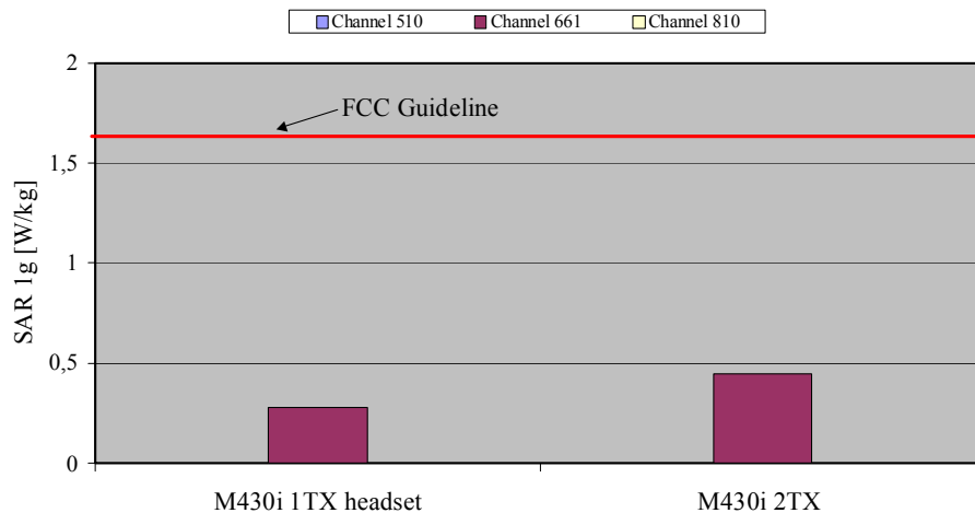
Fig. 8: The measured head phantom SAR values for the Mitsubishi 430i for PCS 1900 in comparison to the FCC exposure limit.
