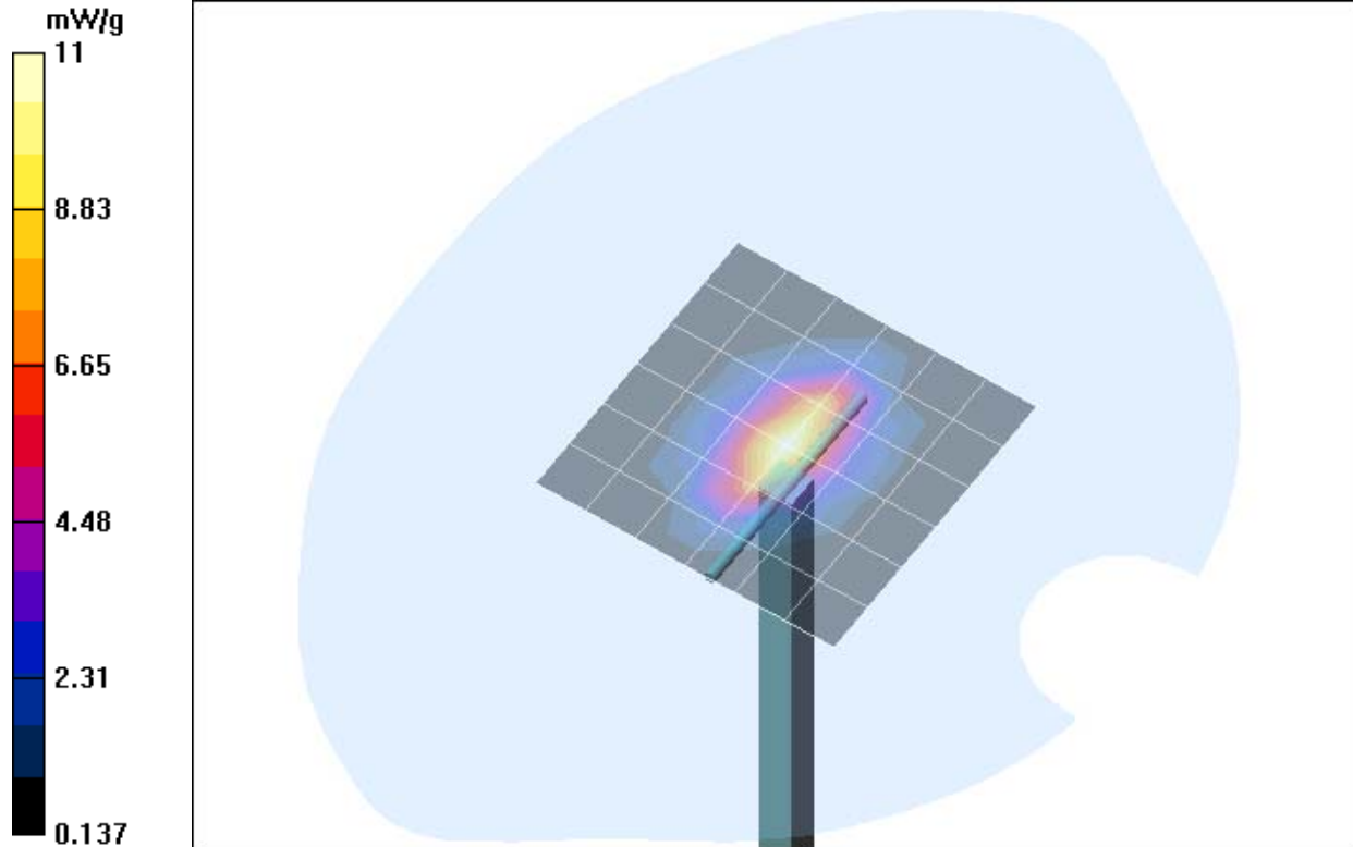
Fig. 10: Validation measurement 1900 MHz Head (September 03, 2004, coarse grid. Ambient Temperature: 21.3° C, Liquid Temperature: 20.7° C).
