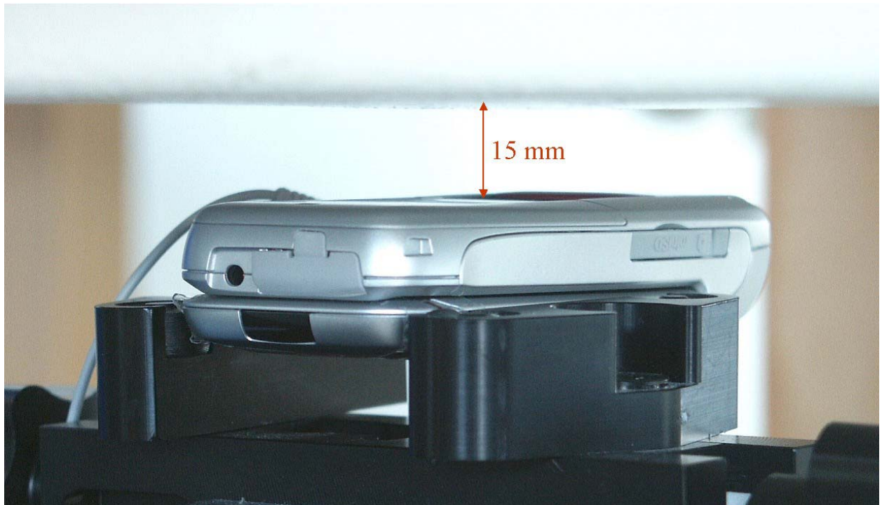
Fig. 20: Body worn configuration, GSM mode (1 TX ) with headset, antenna towards the phantom.
