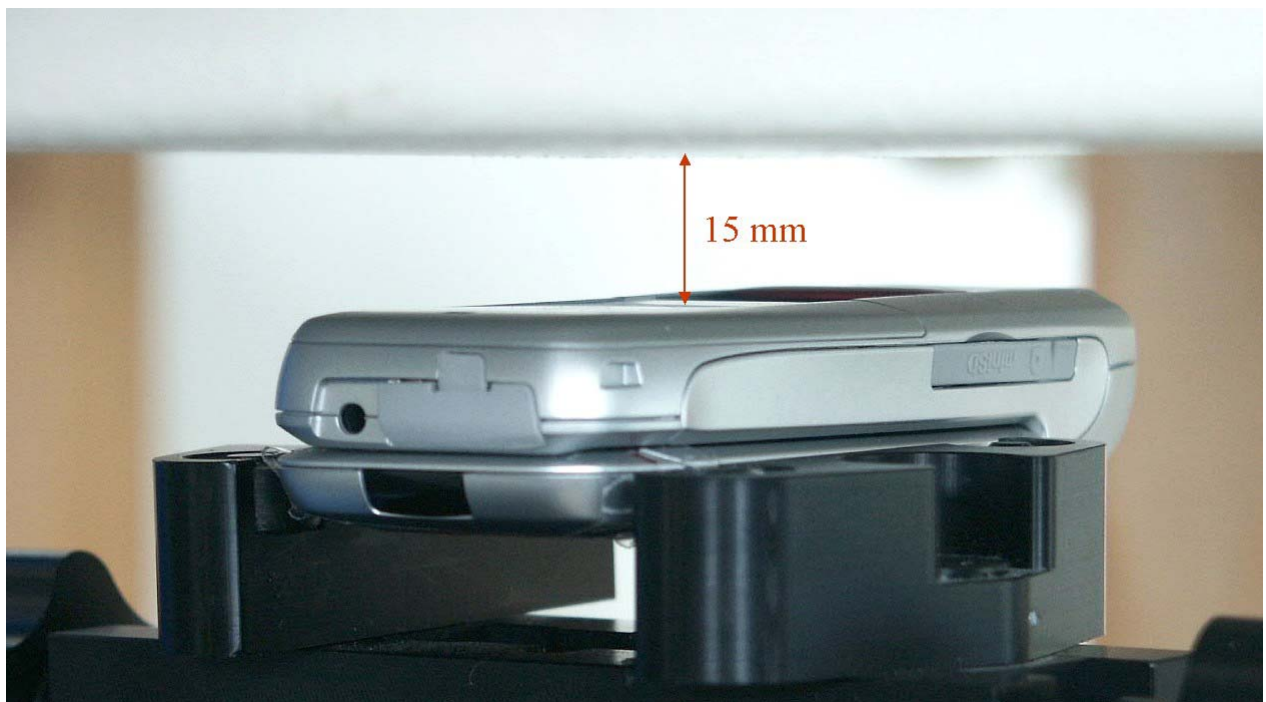
Fig. 21: Body worn configuration, GPRS mode (2 TX slot), antenna towards the phantom.
