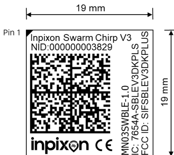
Figure 11-2: Label dimensions (not to scale)
