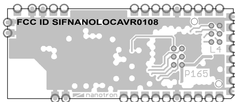
Figure 2: nanoLOC AVR Module - bottom side showing FCC label location
