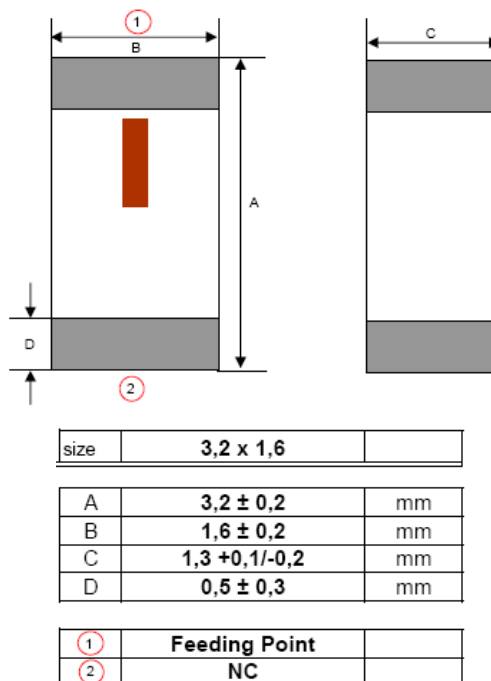
Figure 1: SMD Antenna WE-MCA
