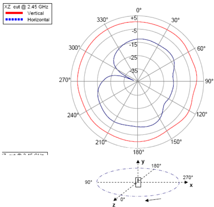
Figure 7: Radiation patterns - XZ cut scanning direction
