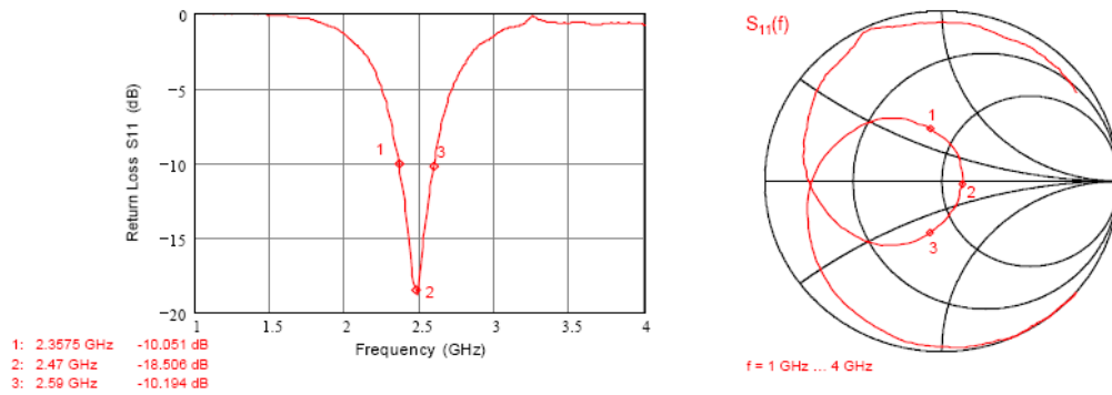
Figure 5: Measuring diagram with matching circuits
