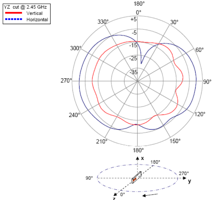
Figure 8: Radiation patterns - YZ cut scanning direction
