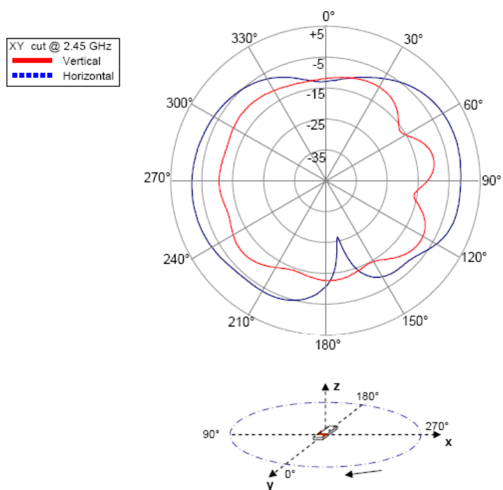
Figure 6: Radiation patterns - XY cut scanning direction
