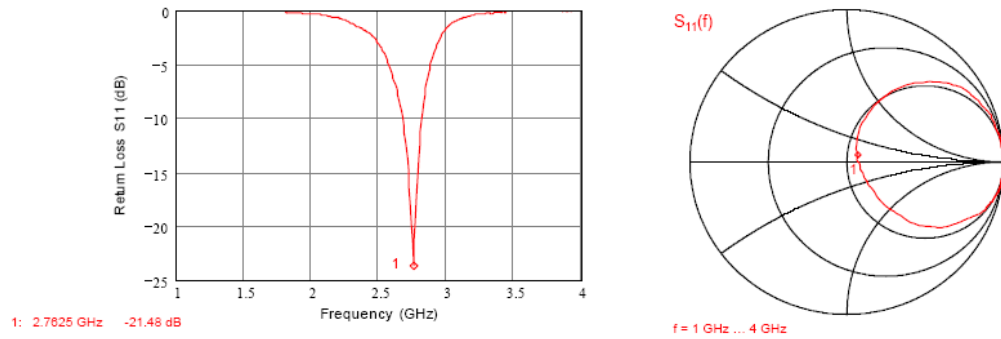
Figure 4: Measuring diagram without matching circuits
