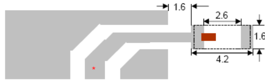
Figure 2: Solder pads without matching circuits
