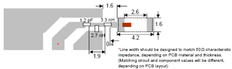
Figure 3: Solder pads with matching circuits
