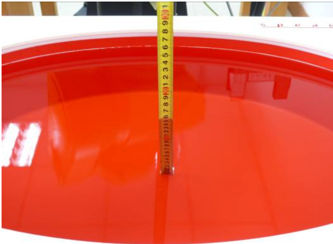
Picture 3: Liquid depth in the flat Phantom (5200 MHz, 15.4cm depth)
