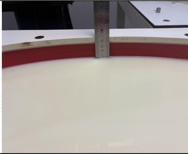
Photo 1: Tissue Simulant Liquid for Head 700-3000
