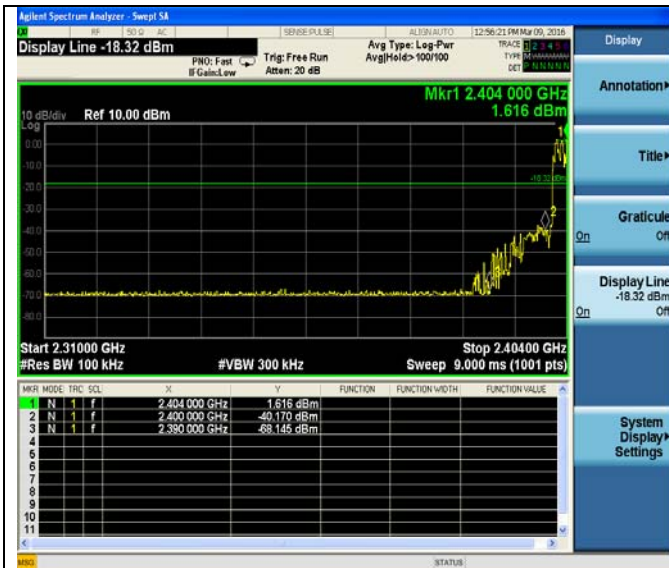
Hopping On- 8-DPSK-Low channel
