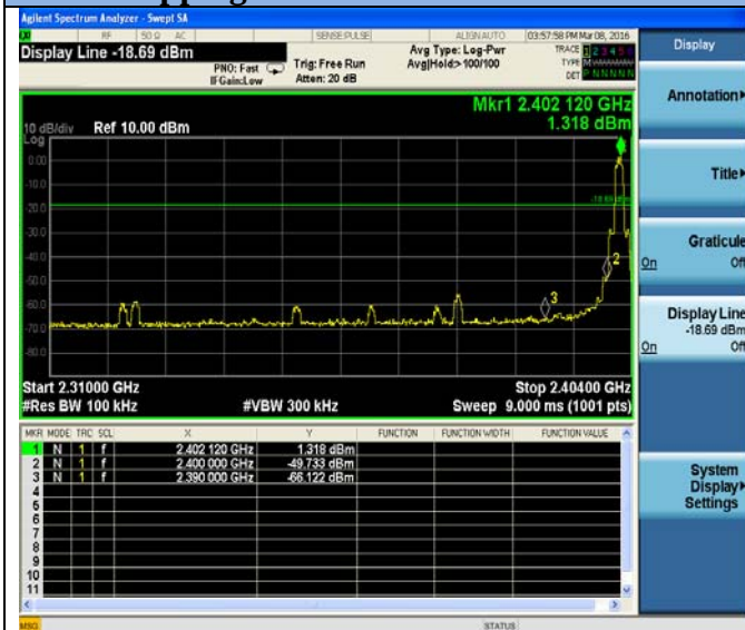
Hopping Off- 8-DPSK-Low channel
