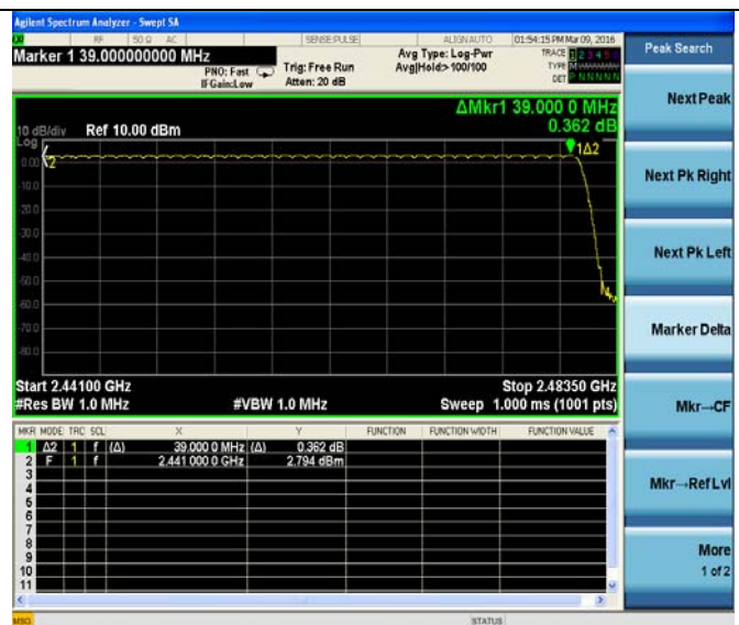
Test Plot 2 For Number of Hopping Channel(GFSK)
